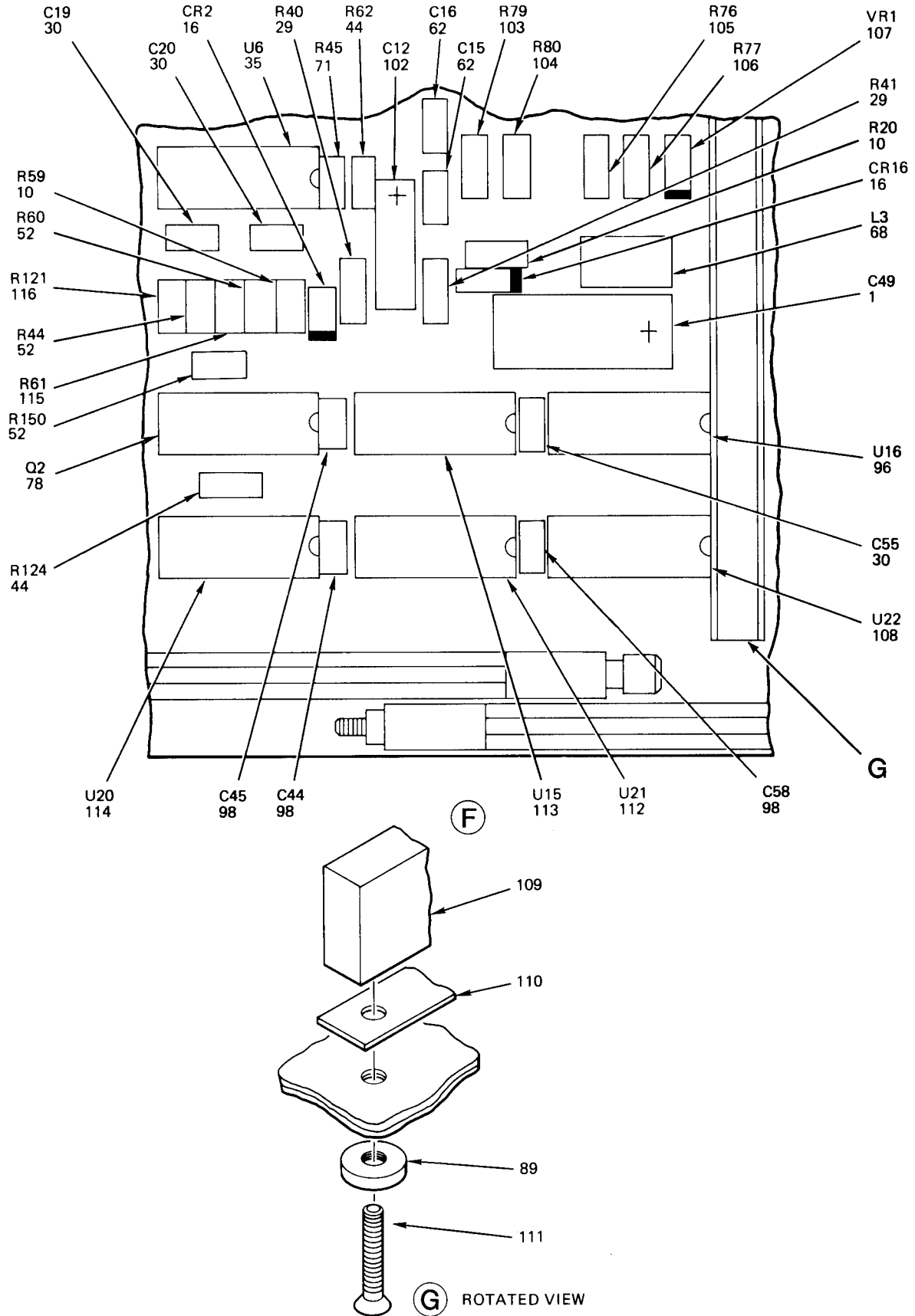
Figure 50. Circuit Card Assembly, Sequence Monitor (Sheet 5 of 6)
