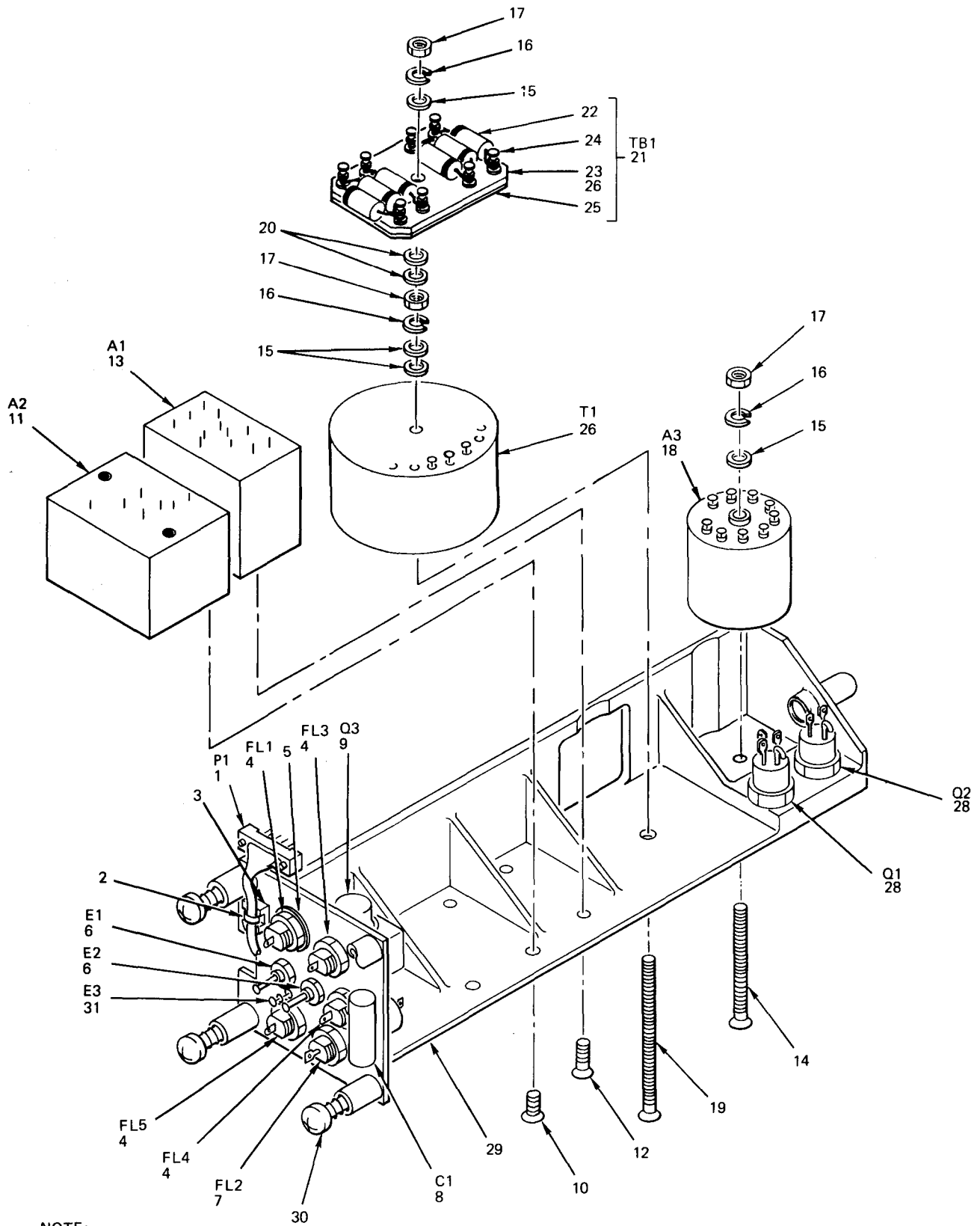
Figure 26. DC/DC Converter Assembly
