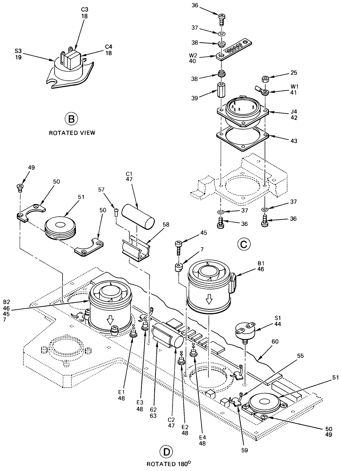
Figure 4. Upper Inertial Measurement Unit Subassembly (Sheet 3 of 4)
