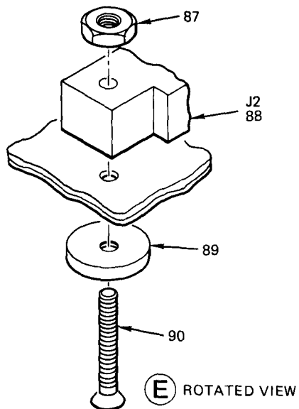
Figure 50. Circuit Card Assembly, Sequence Monitor (Sheet 4 of 6)
