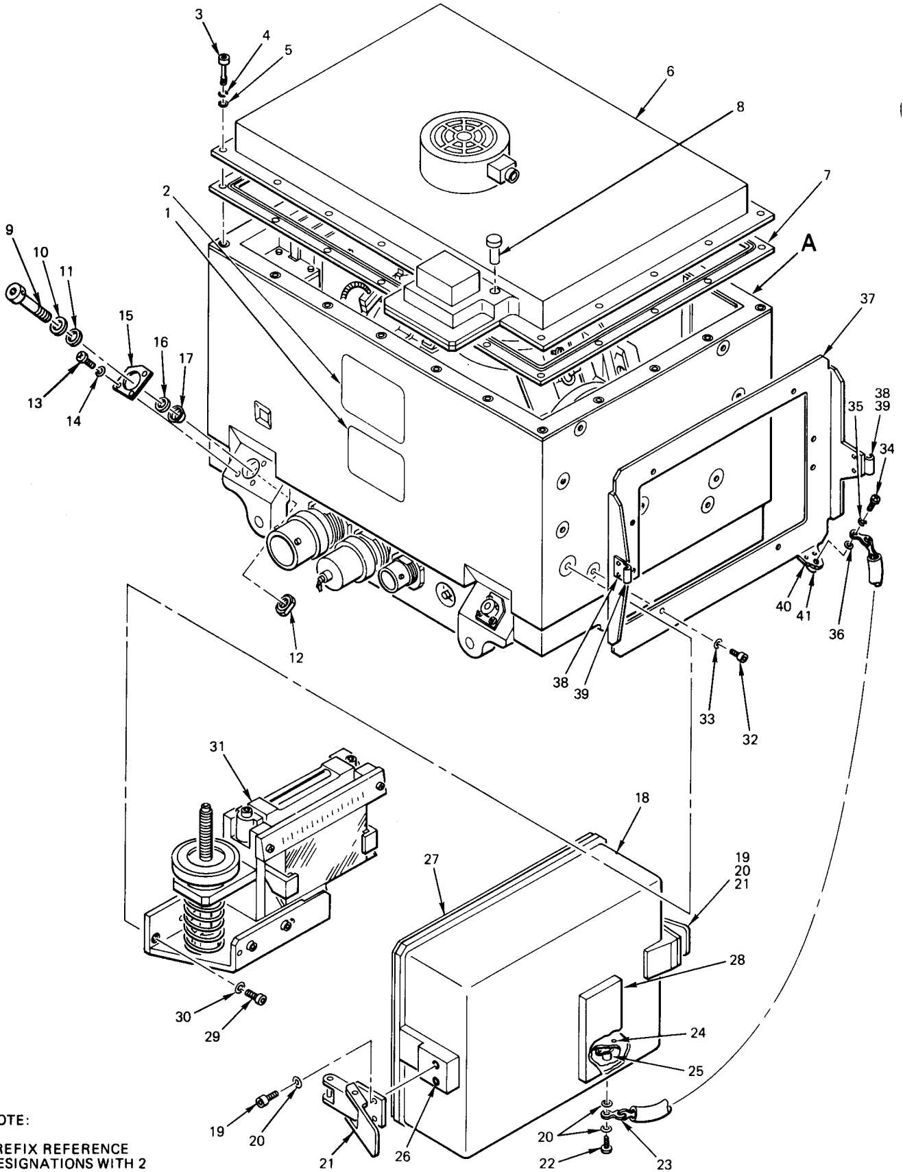
Figure 3. Inertial Measurement Unit (Sheet 1 of 3)
