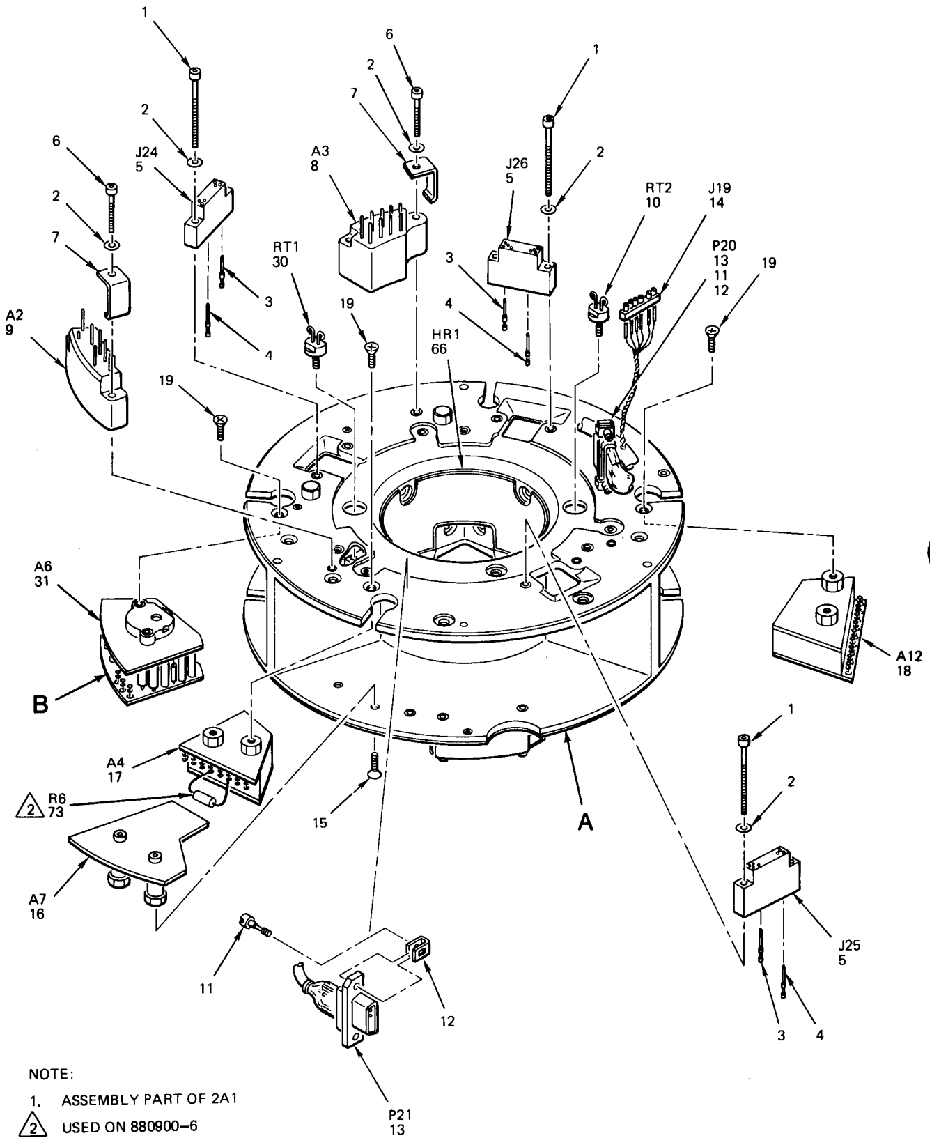
Figure 16. Stable Element Subassembly (Sheet 1 of 3)
