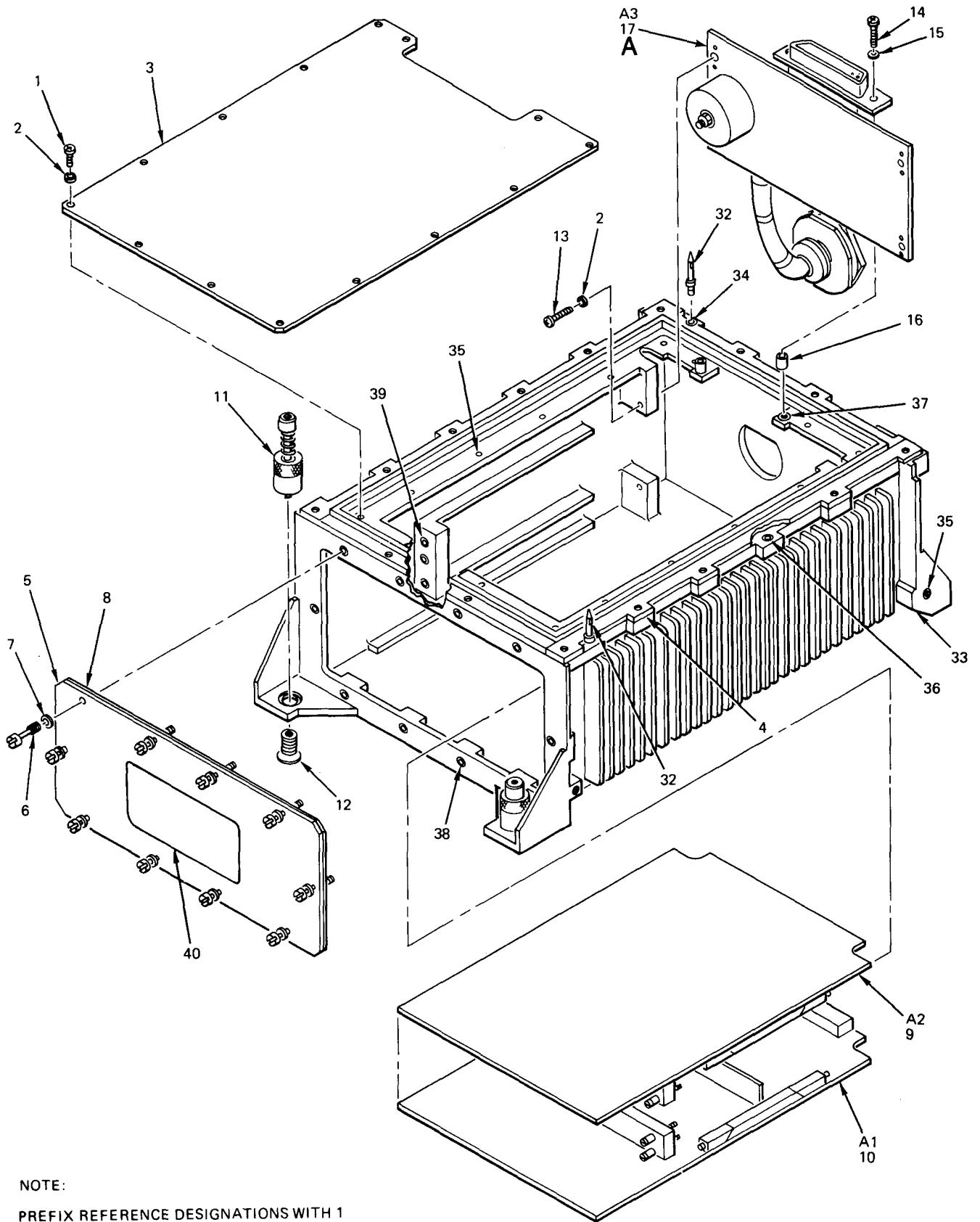
Figure 41. Computer Power Supply (Sheet 1 of 2)
