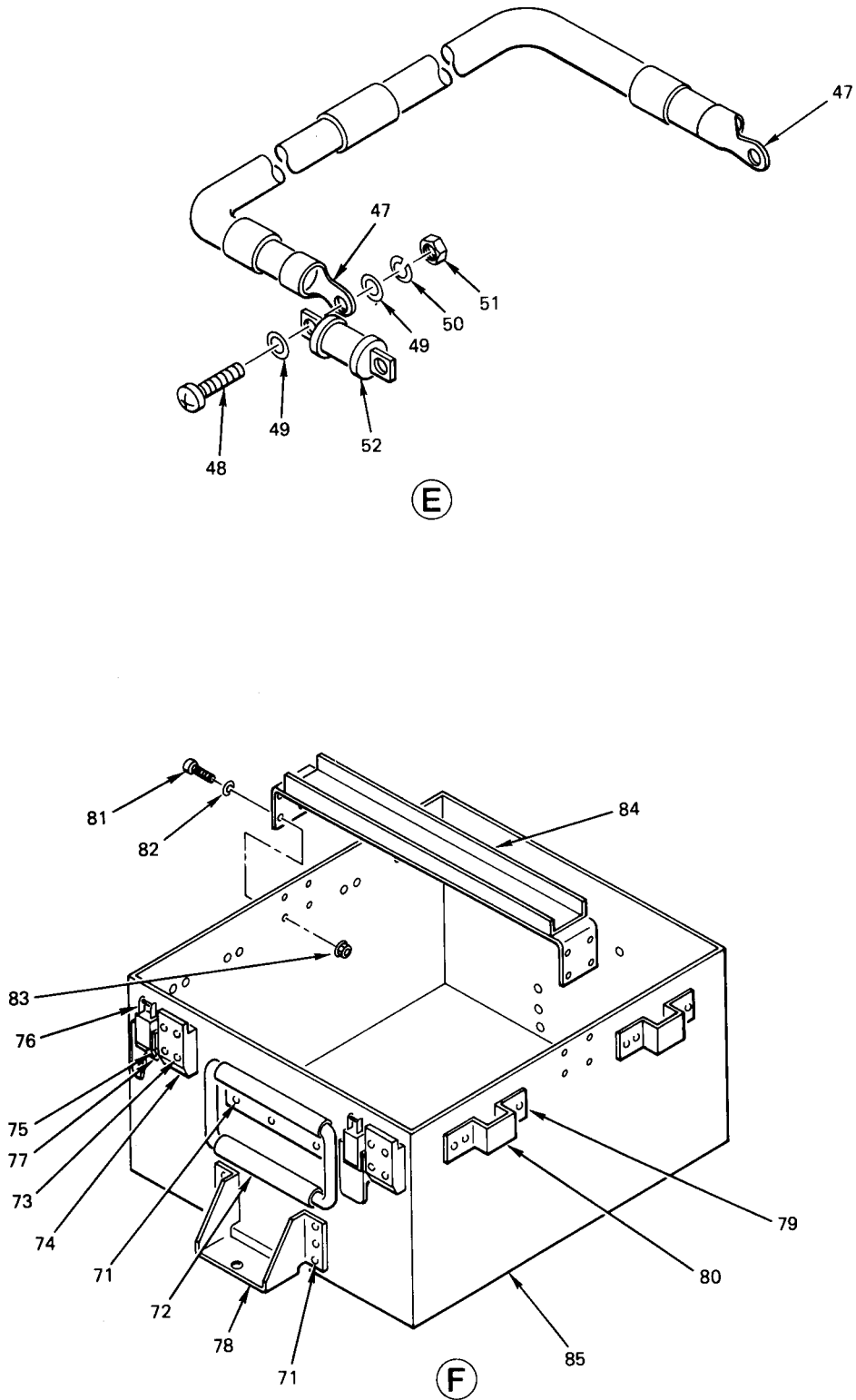
Figure 60. Battery Box (Sheet 5 of 5)
