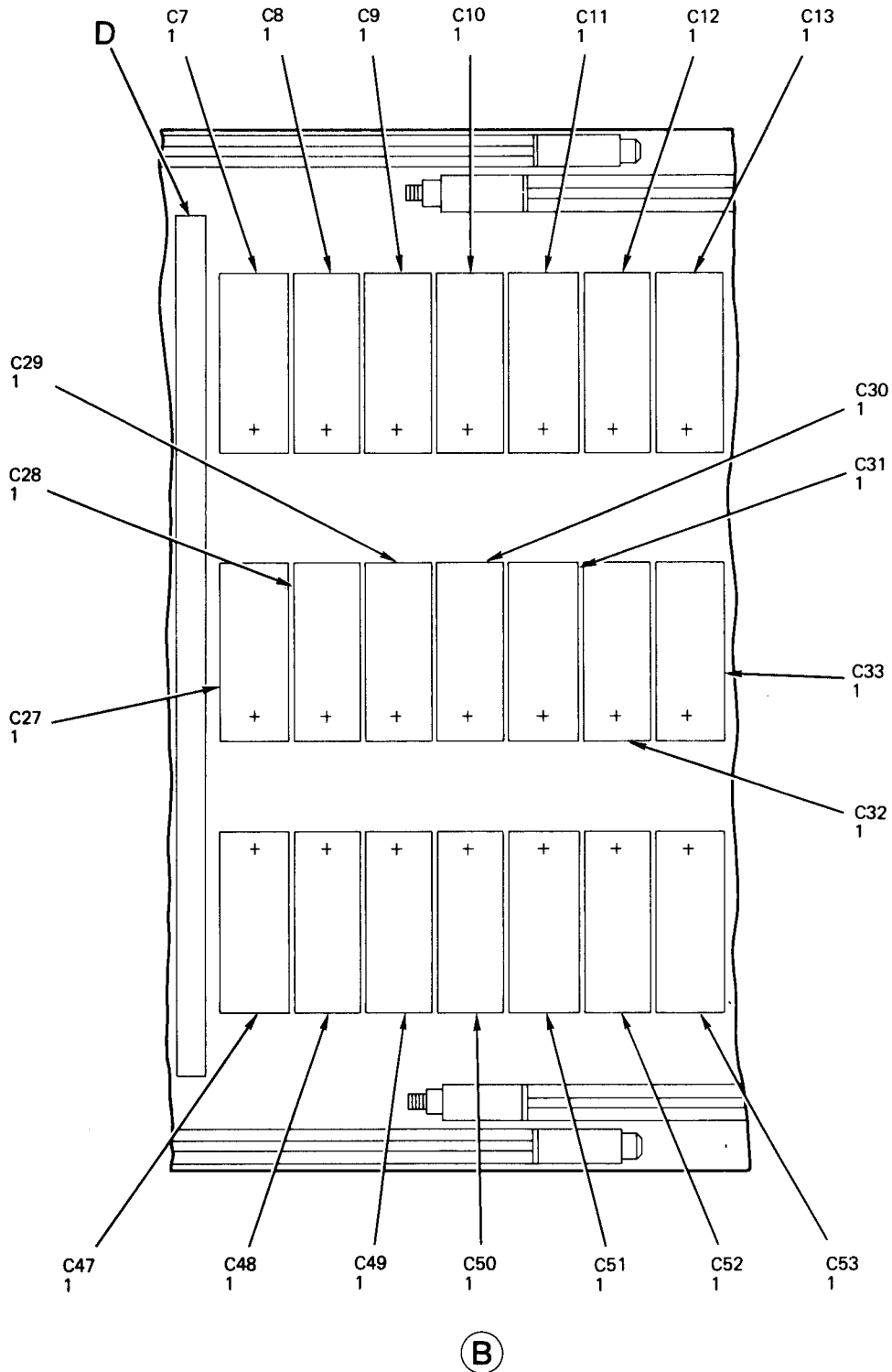
Figure 51. Circuit Card Assembly, Filter (Sheet 2 of 4)
