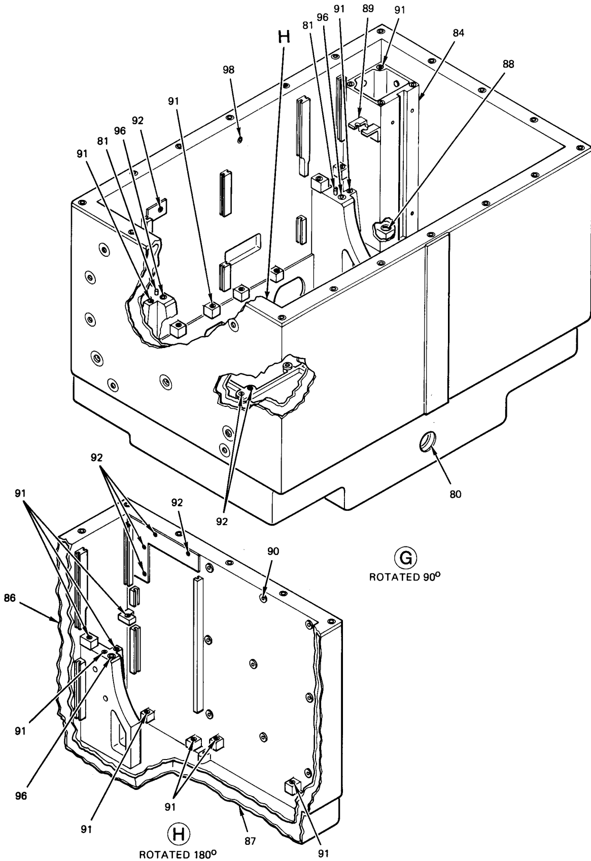
Figure 23. Inertial Measurement Unit Subassembly (Sheet 6 of 6)
