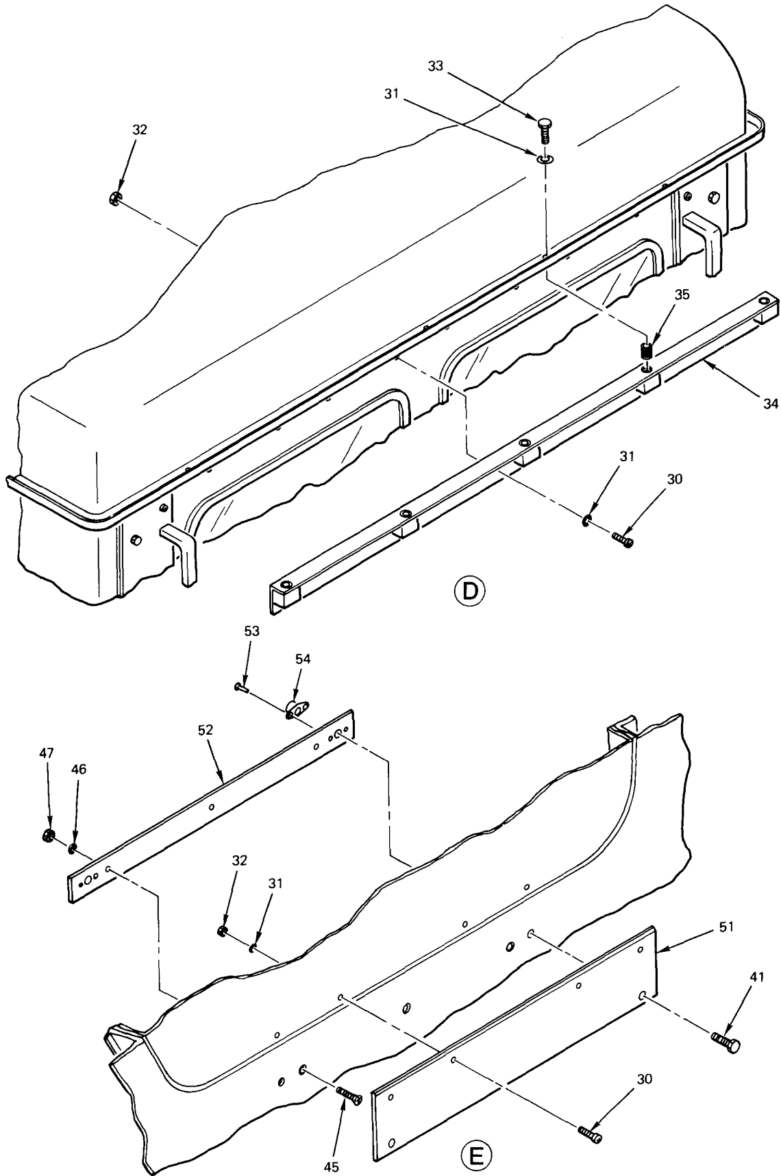
Figure 62. Winterization Kit (Sheet 3 of 4)
