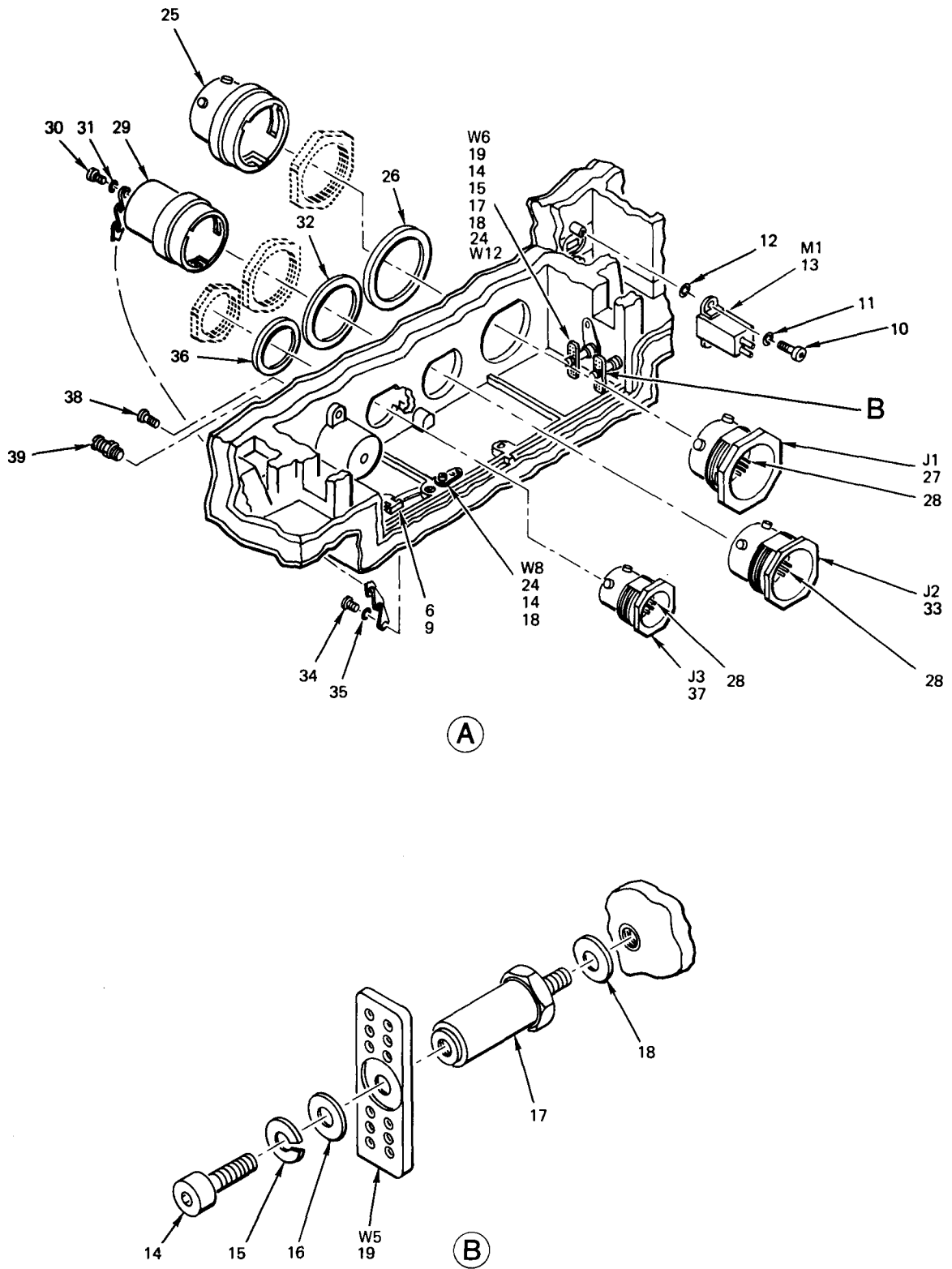
Figure 23. Inertial Measurement Unit Subassembly (Sheet 2 of 6)
