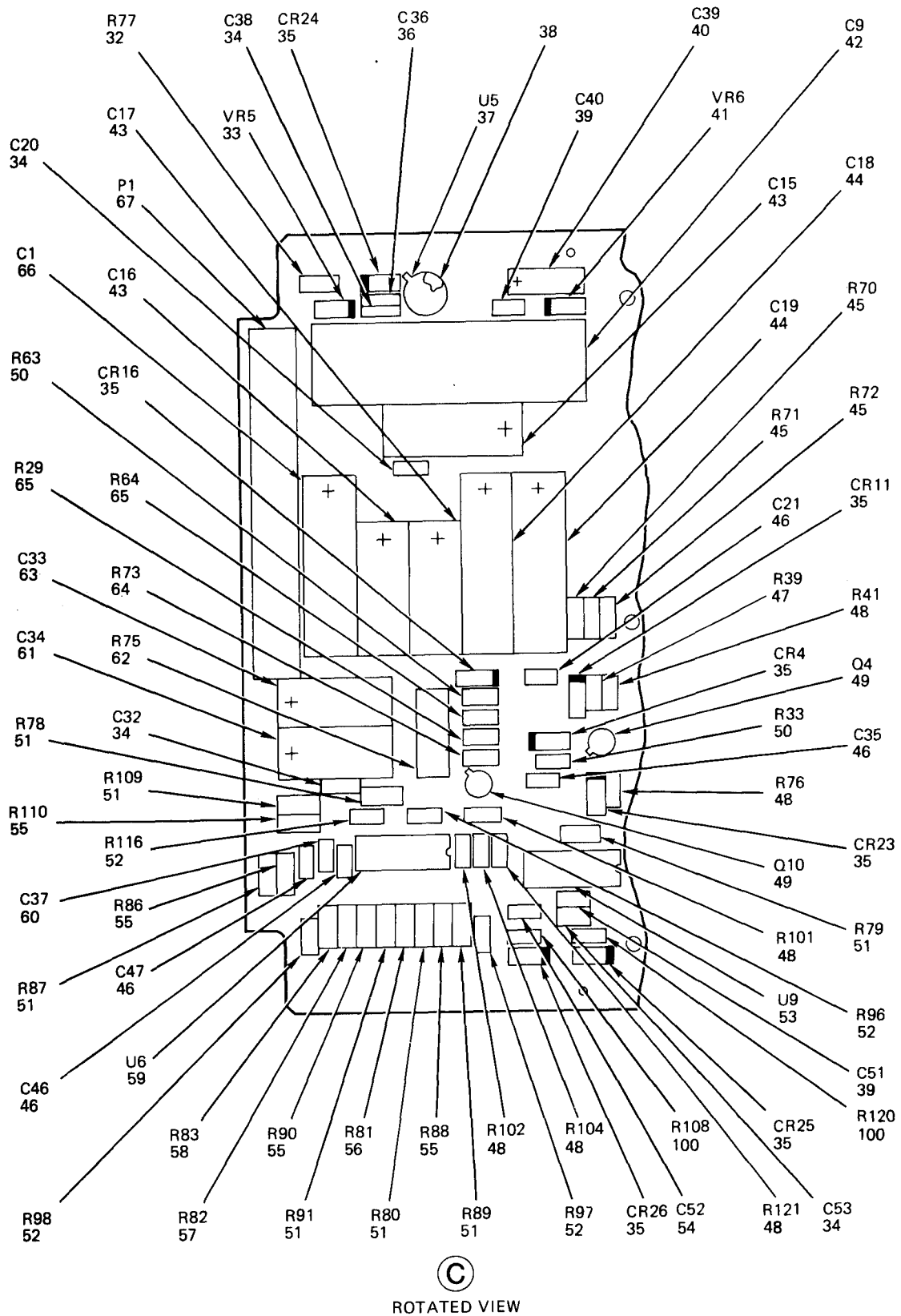
Figure 42. Circuit Card Assembly, 15V (Sheet 2 of 4)
