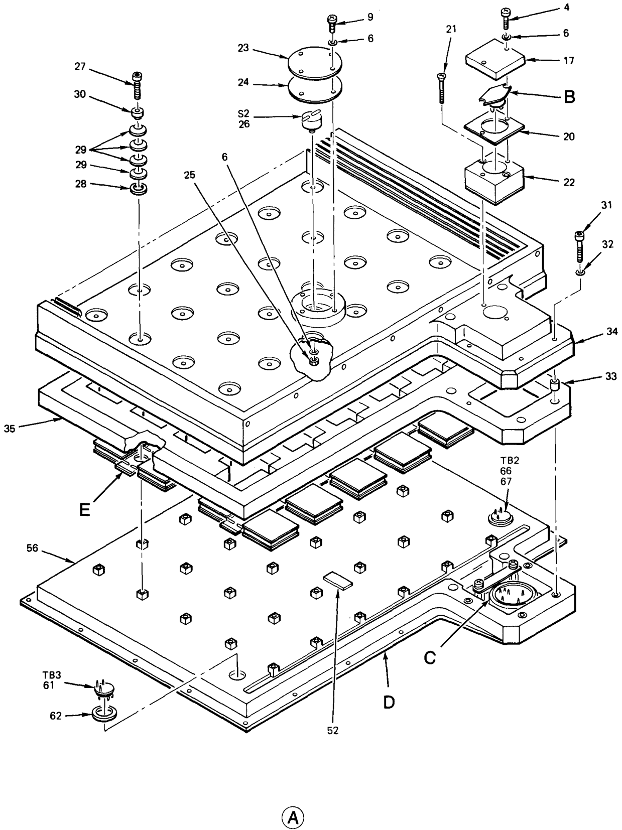
Figure 4. Upper Inertial Measurement Unit Subassembly (Sheet 2 of 4)
