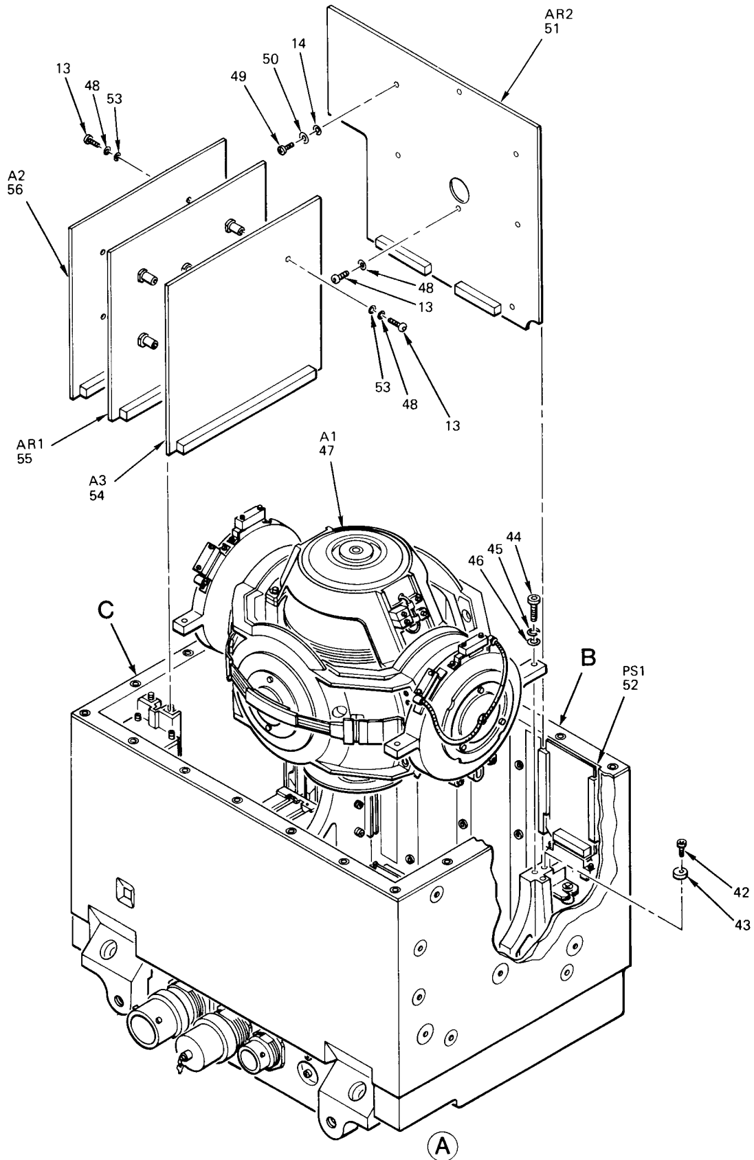
Figure 3. Inertial Measurement Unit (Sheet 2 of 3)
