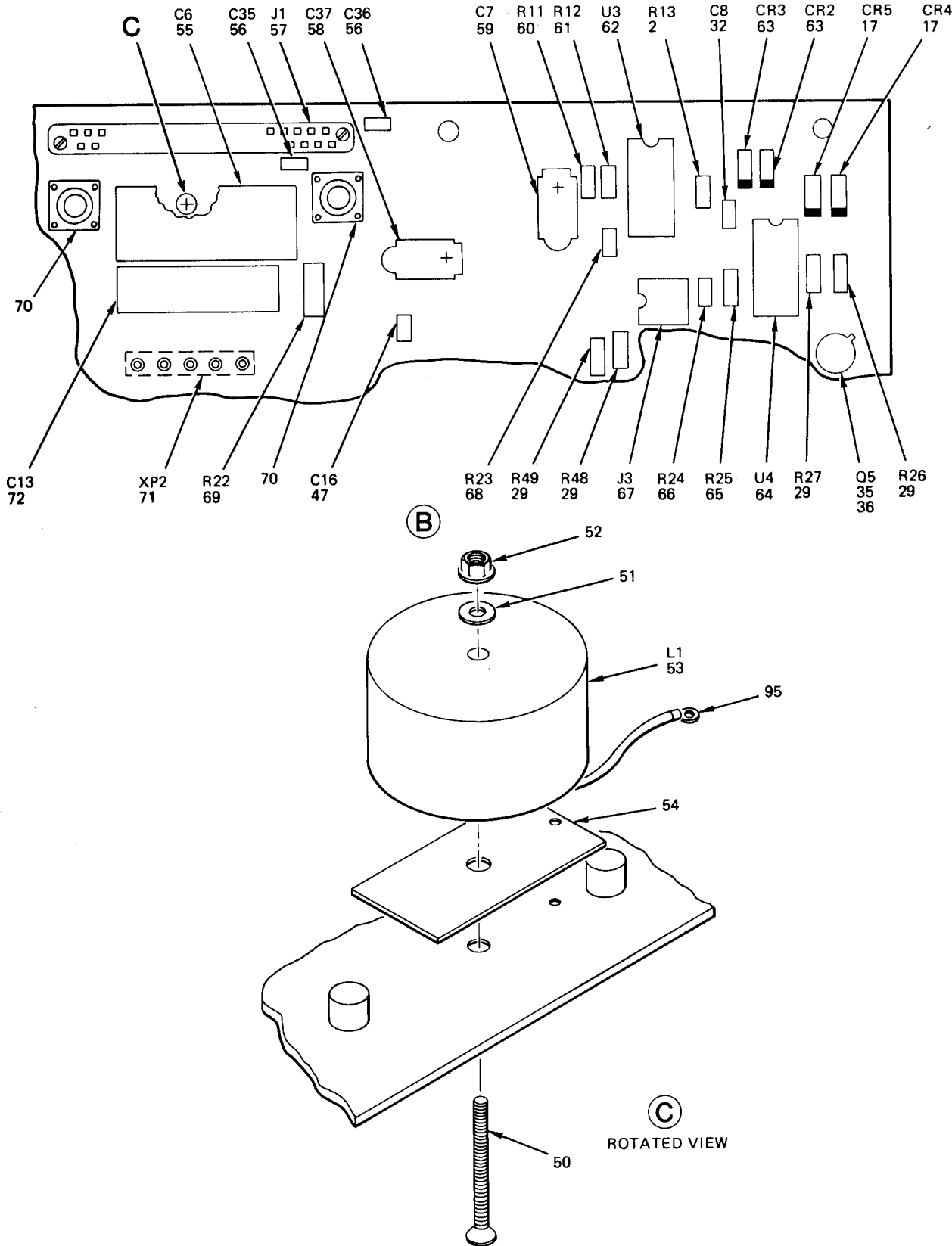
Figure 46. Circuit Card Assembly, Power Inverter (Sheet 2 of 4)
