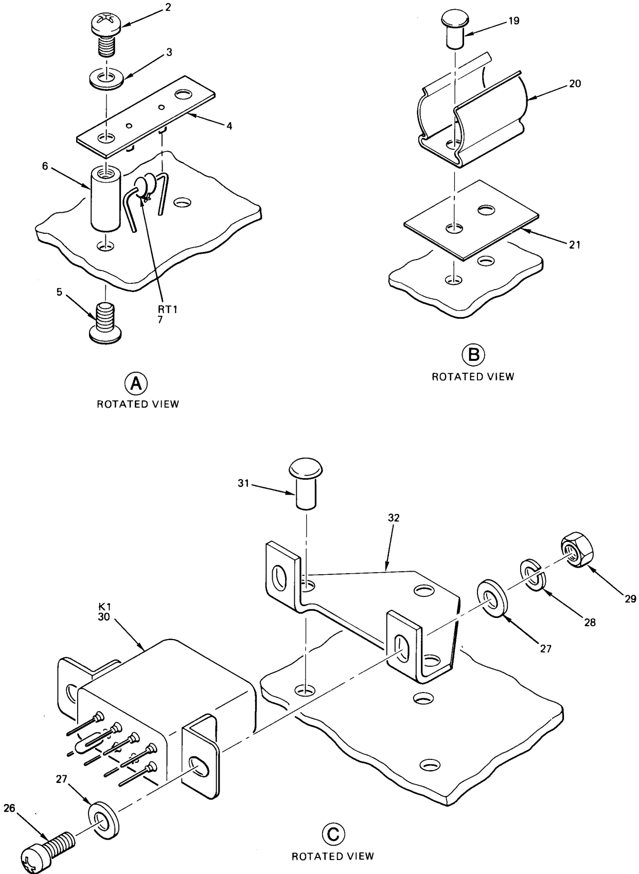
Figure 24. Circuit Card Assembly, Ambient Temperature Control (Sheet 2 of 2)
