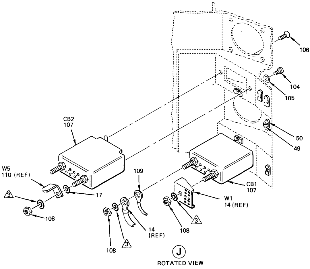
Figure 53. Power Supply Subassembly (Sheet 5 of 6)
