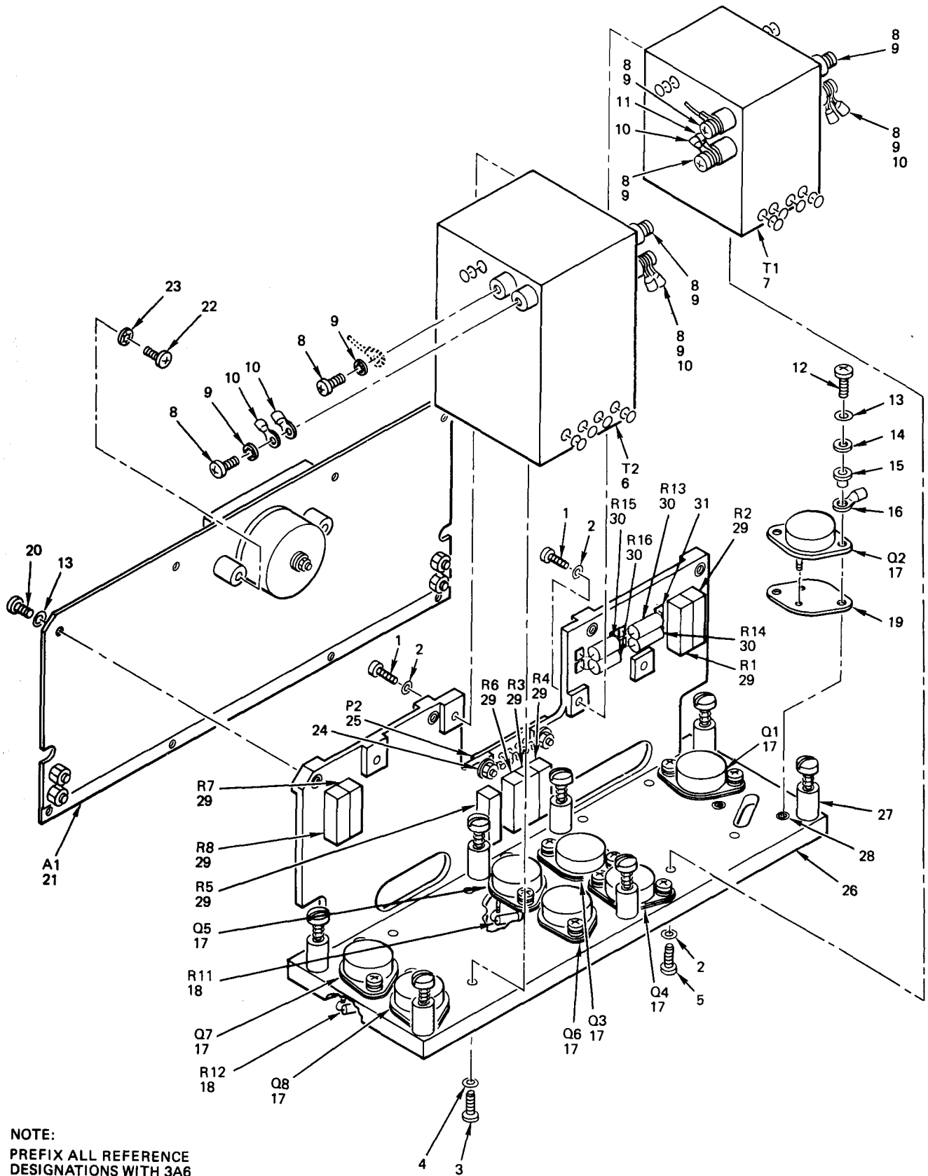
Figure 45. Inverter Assembly
