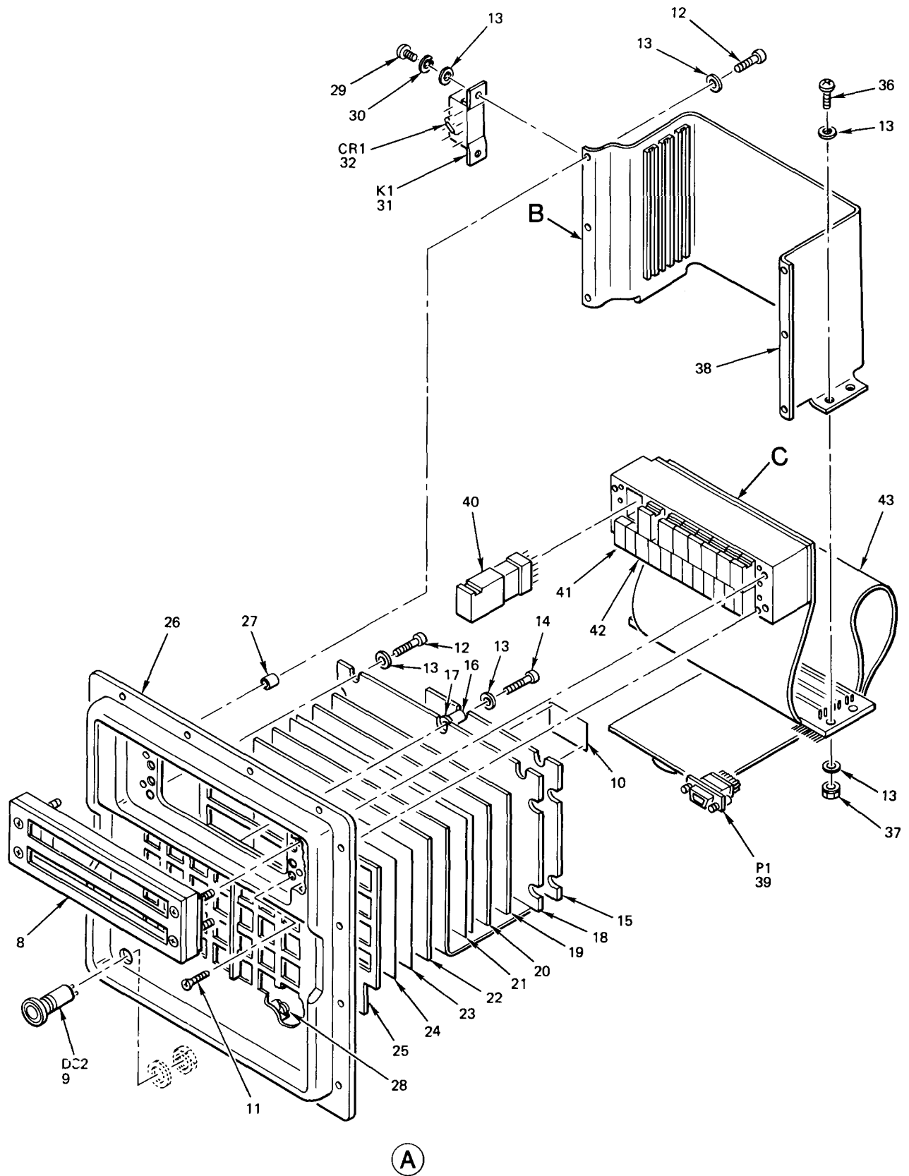
Figure 57. Control and Display Unit (Sheet 2 of 3)
