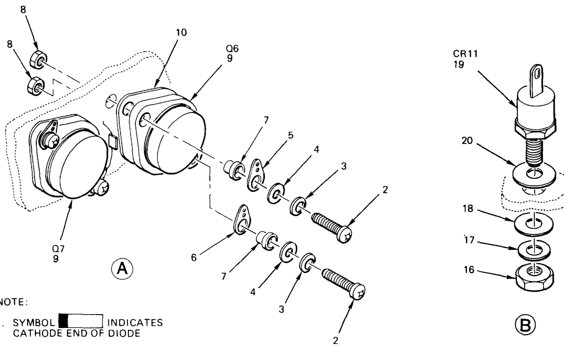
Figure 47. Circuit Card Assembly, Battery Charger (Sheet 1 of 2)
