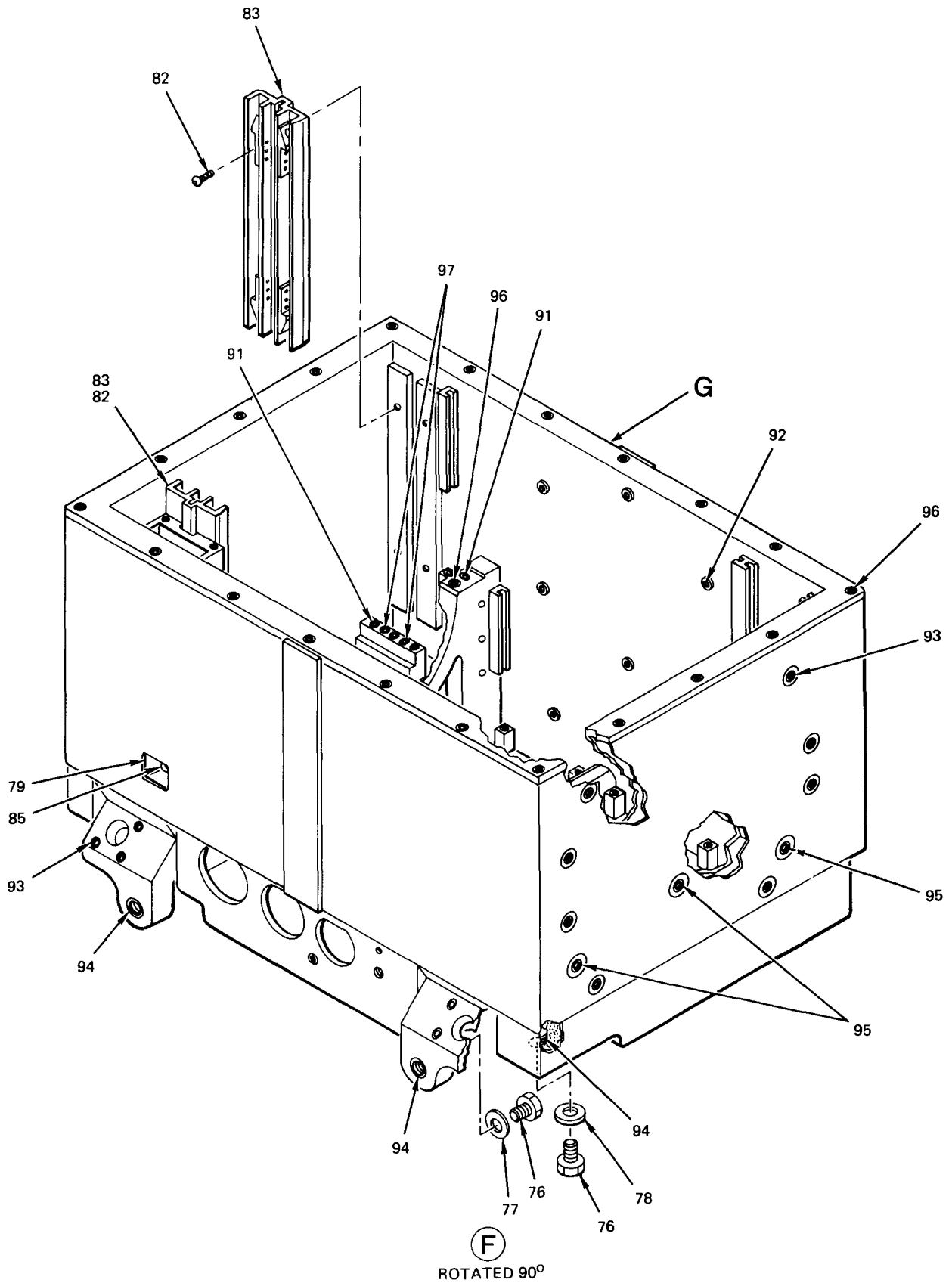
Figure 23. Inertial Measurement Unit Subassembly (Sheet 5 of 6)
