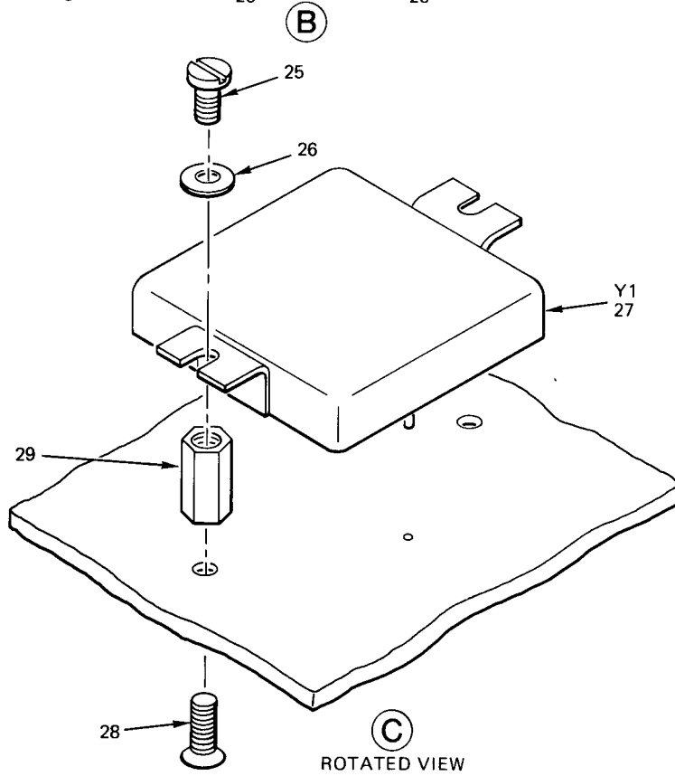
Figure 22. Circuit Card Assembly Mode (Sheet 2 of 2)
