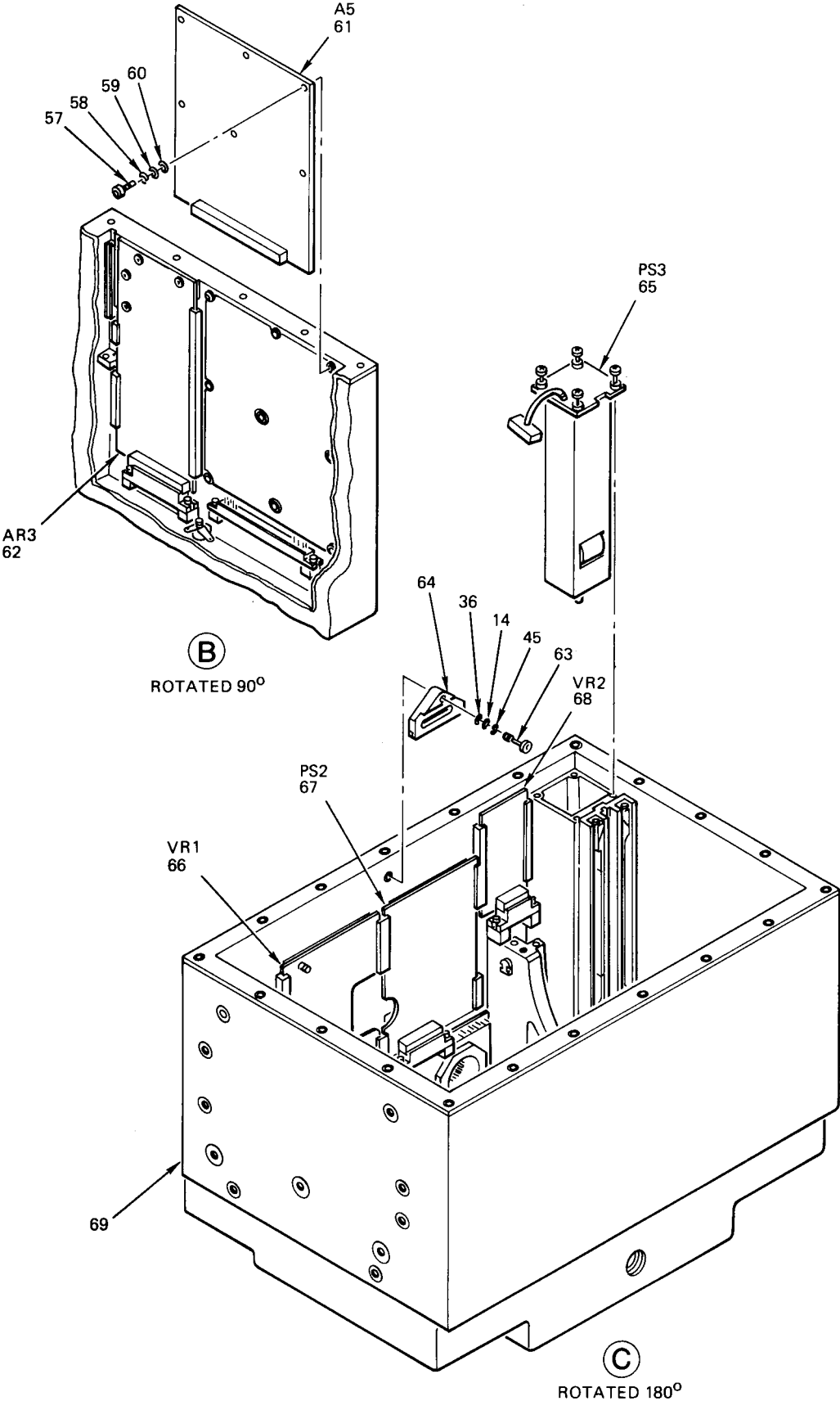
Figure 3. Inertial Measurement Unit (Sheet 3 of 3)
