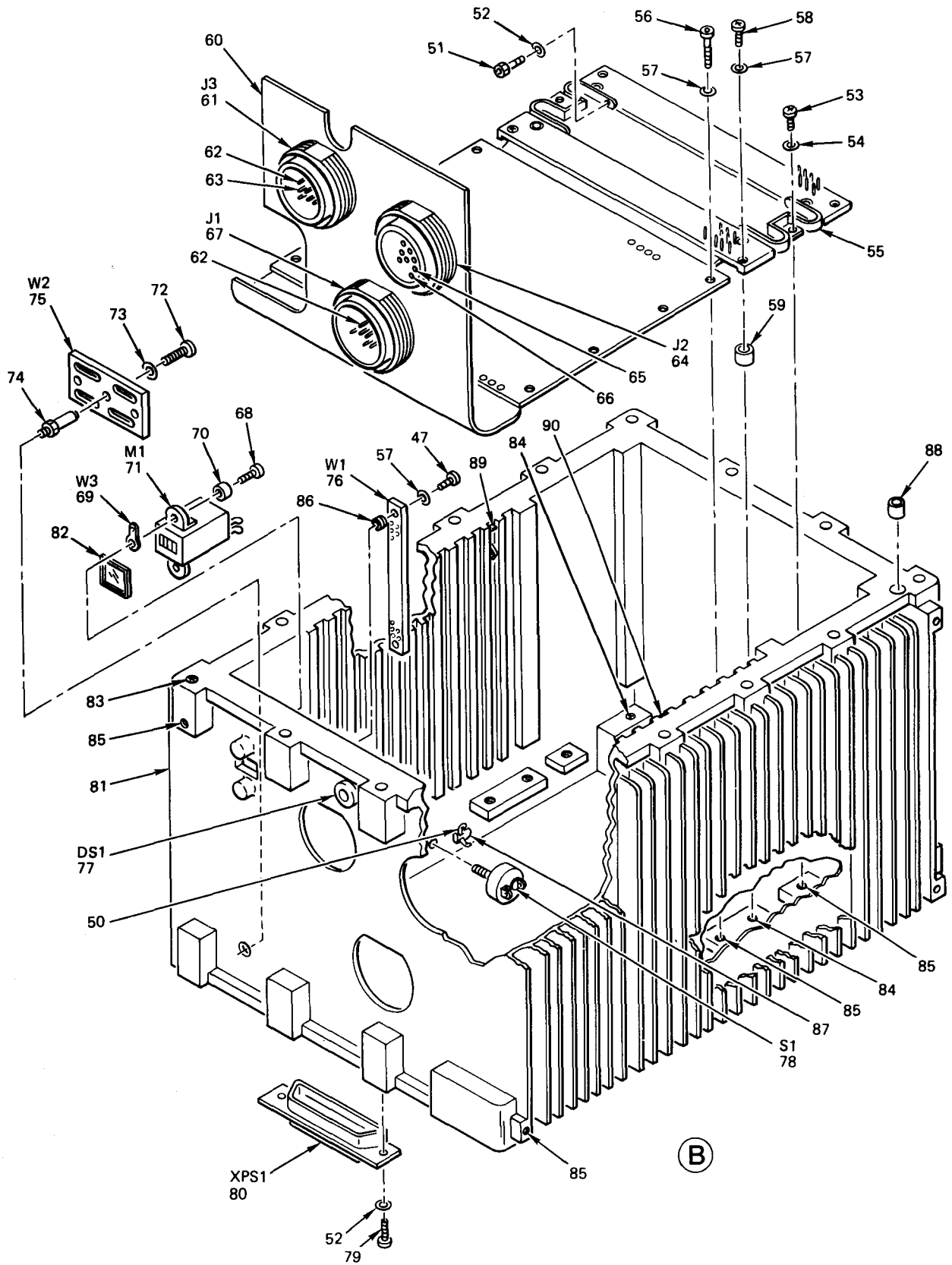
Figure 30. Computer (Sheet 3 of 3)
