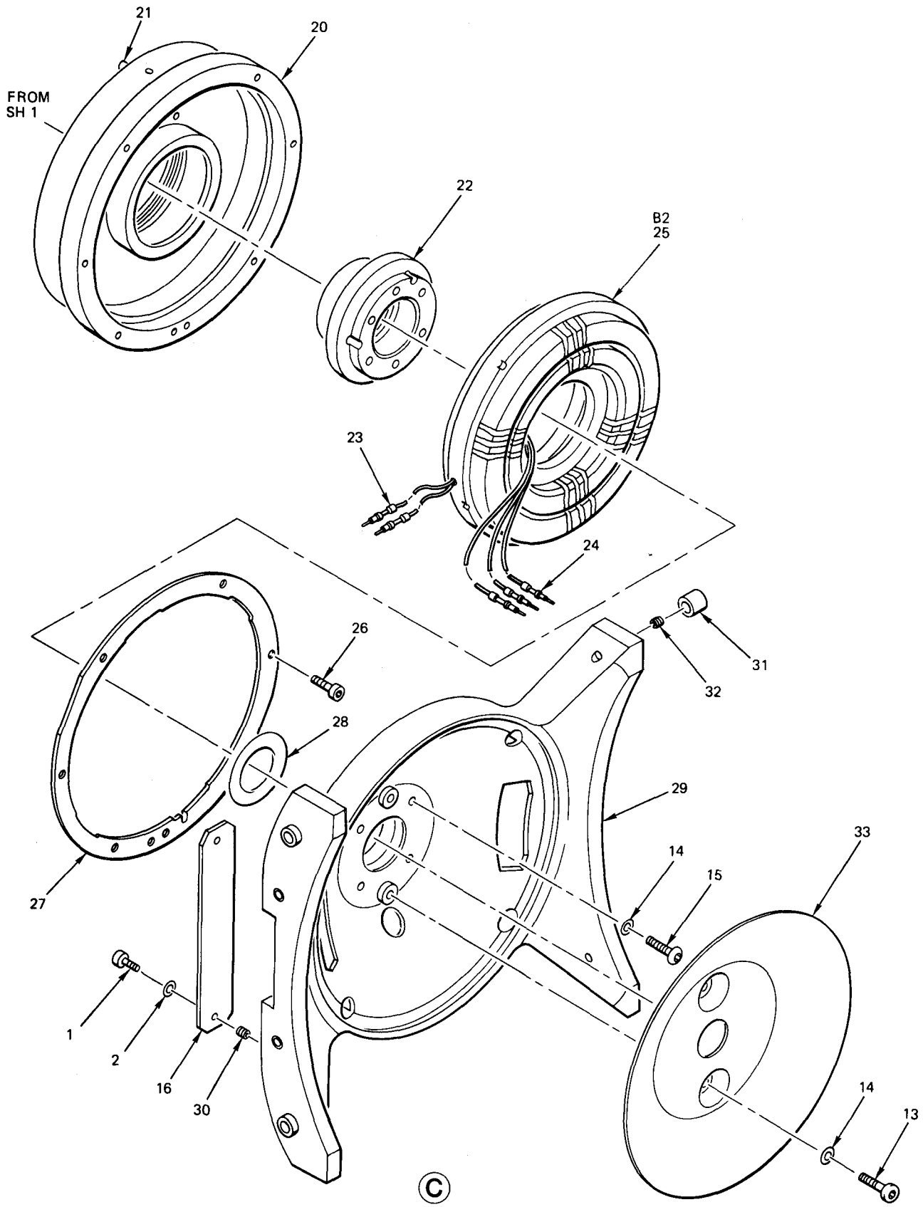
Figure 11. Outer Roll Cartridge Assembly, Resolver (Sheet 2 of 2)
