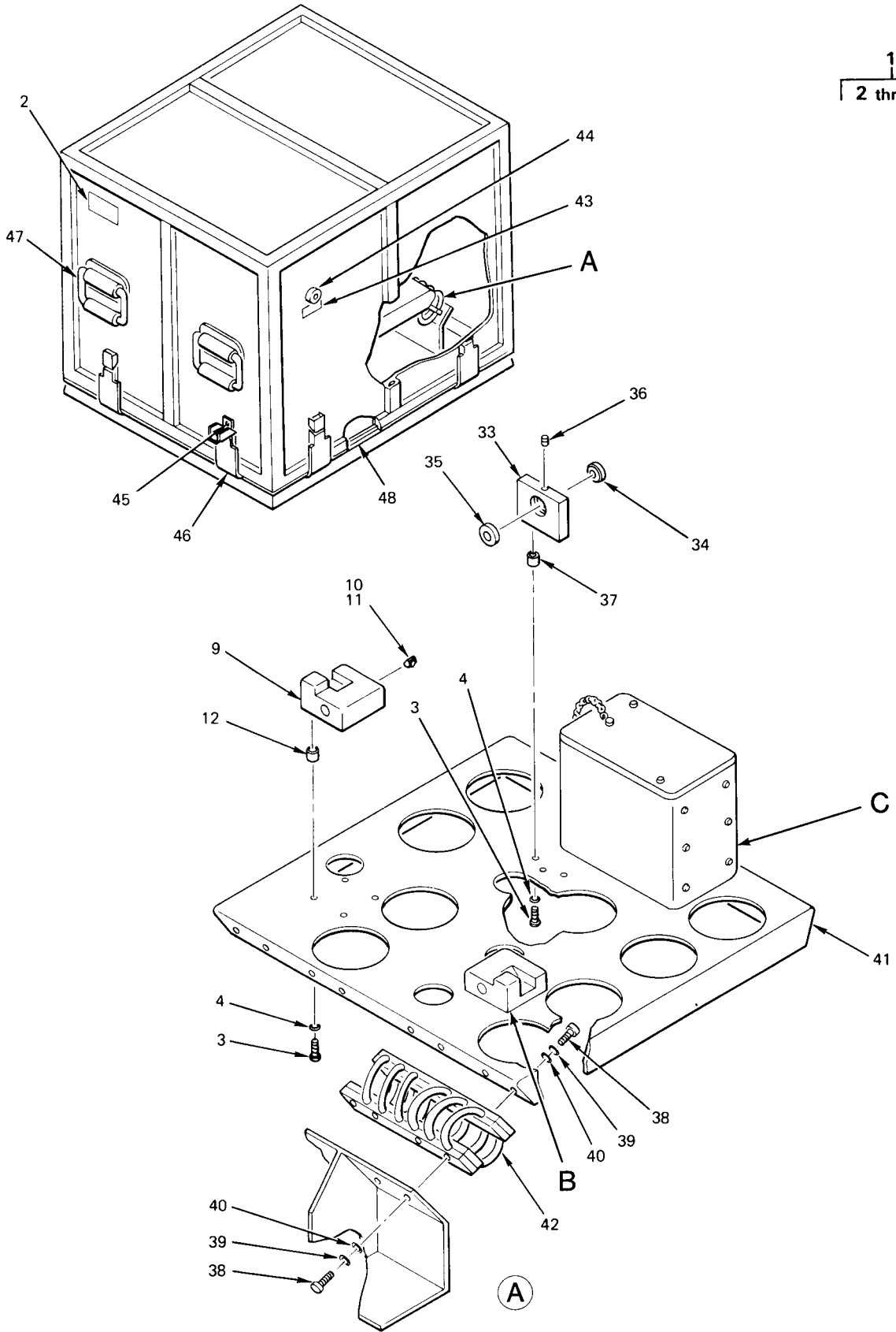
Figure 64. Transit Case, IMU and Memory (Sheet 1 of 2)
