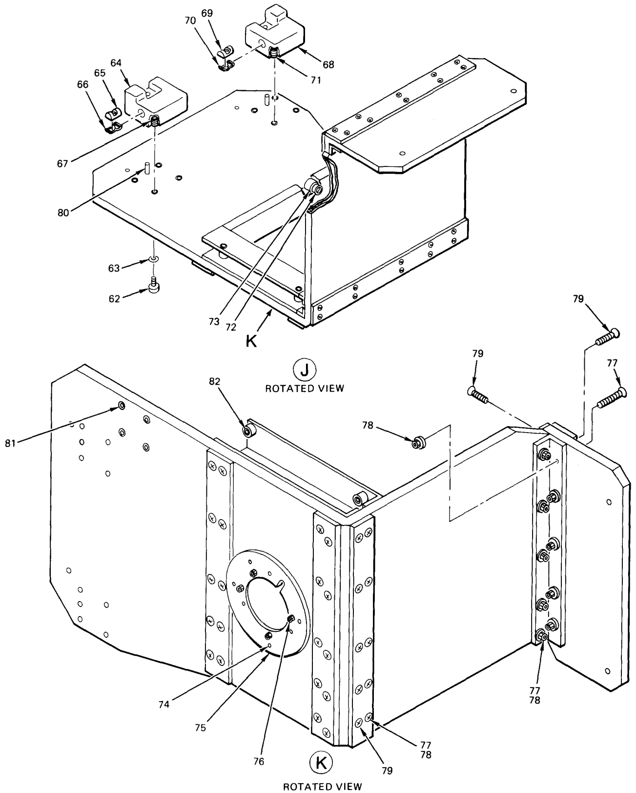
Figure 2. Electrical Equipment Mounting Base (Sheet 4 of 5)
