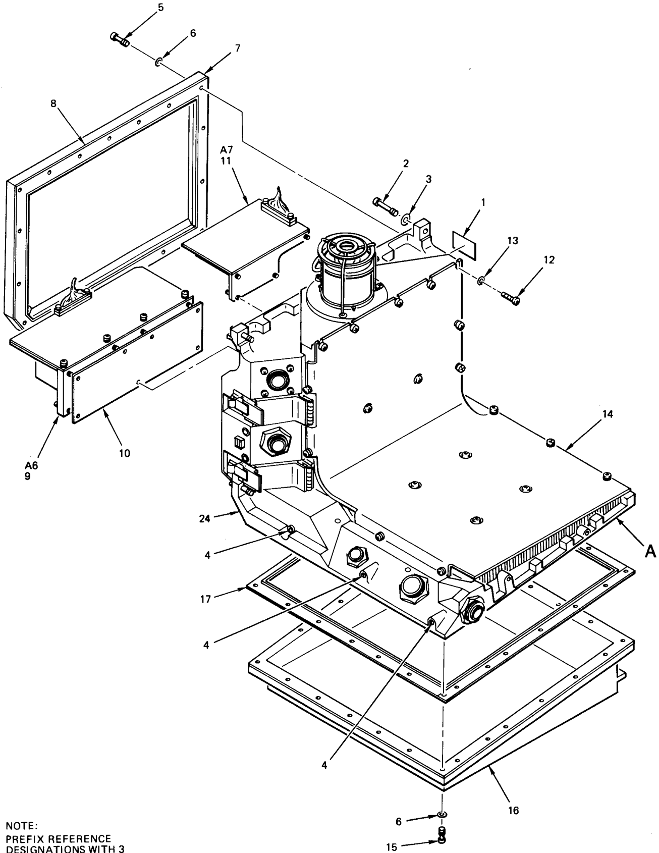
Figure 44. Power Supply (Sheet 1 of 2)
