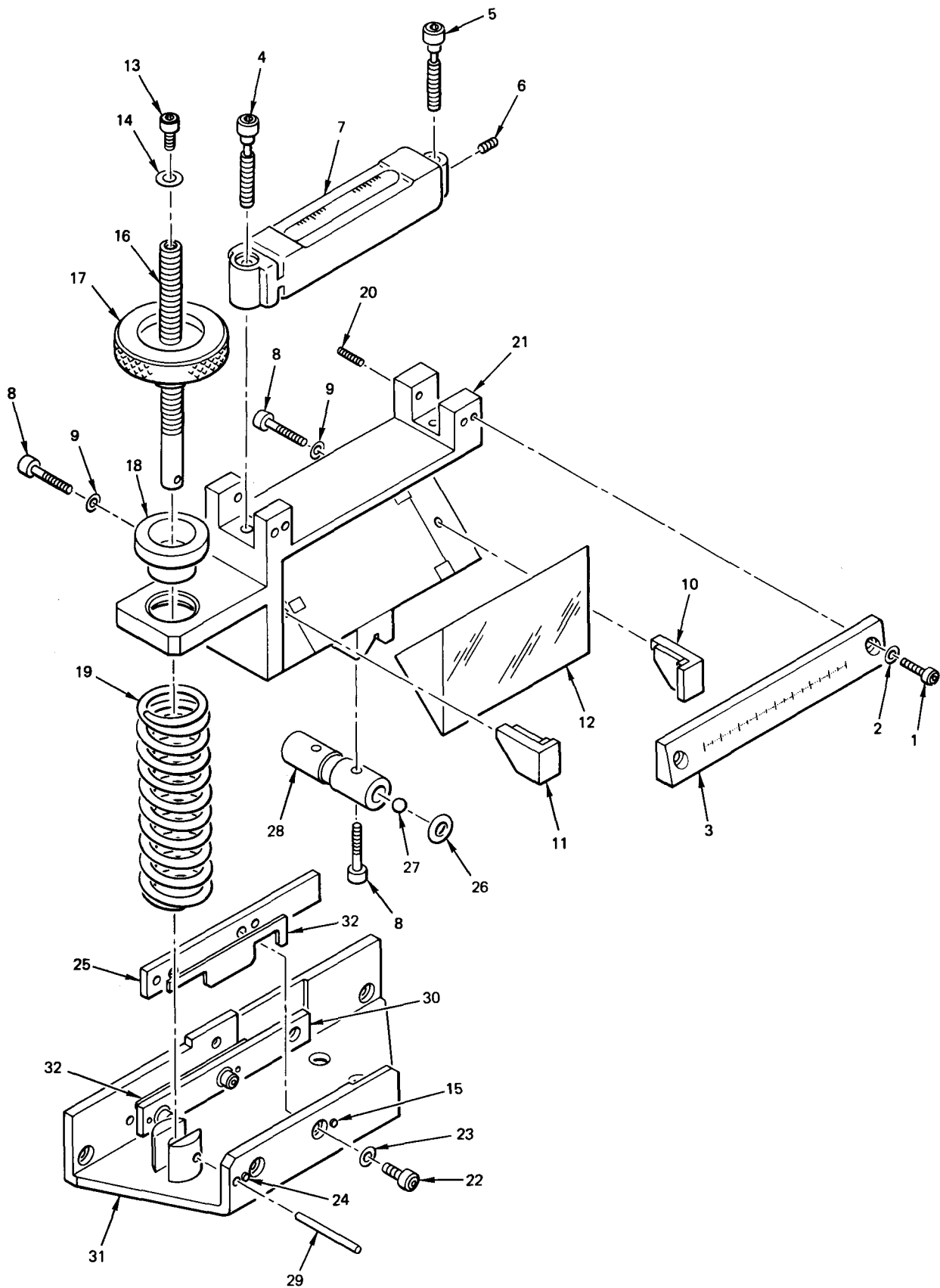
Figure 5. Porro Prism Assembly
