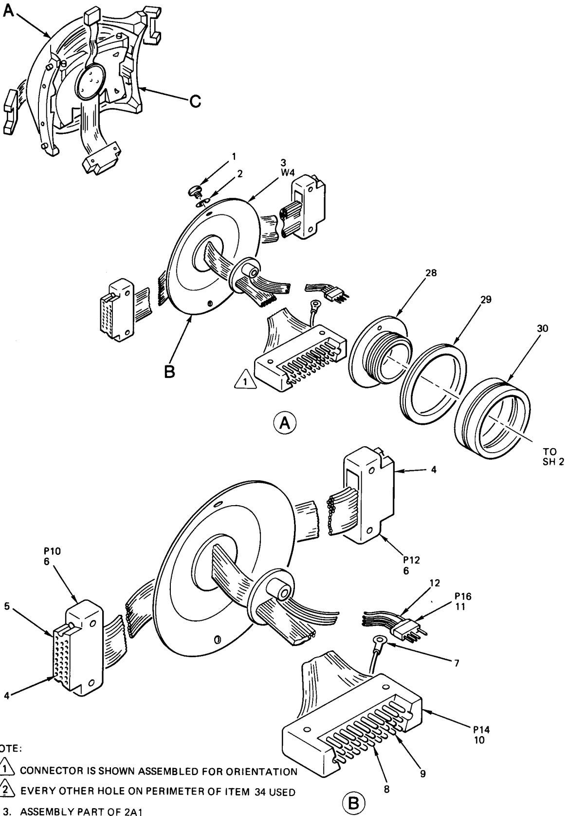
Figure 8. Inner Roll Cartridge Assembly Torquer (Sheet 1 of 3)
