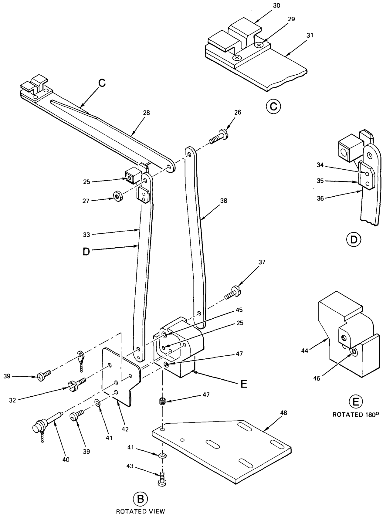
Figure 2. Electrical Equipment Mounting Base (Sheet 2 of 5)
