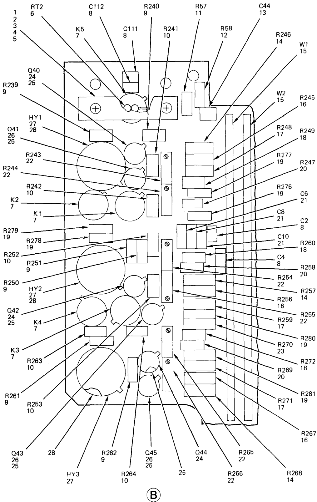
Figure 18. Circuit Card Assembly, Quantizer (Sheet 2 of 8)
