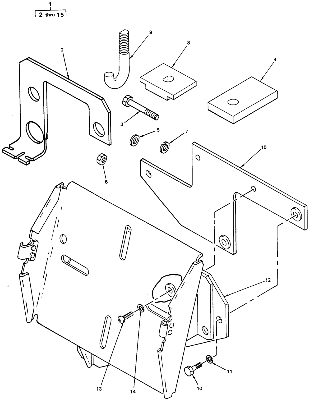
Figure 70. Modification Kit, CUCV
