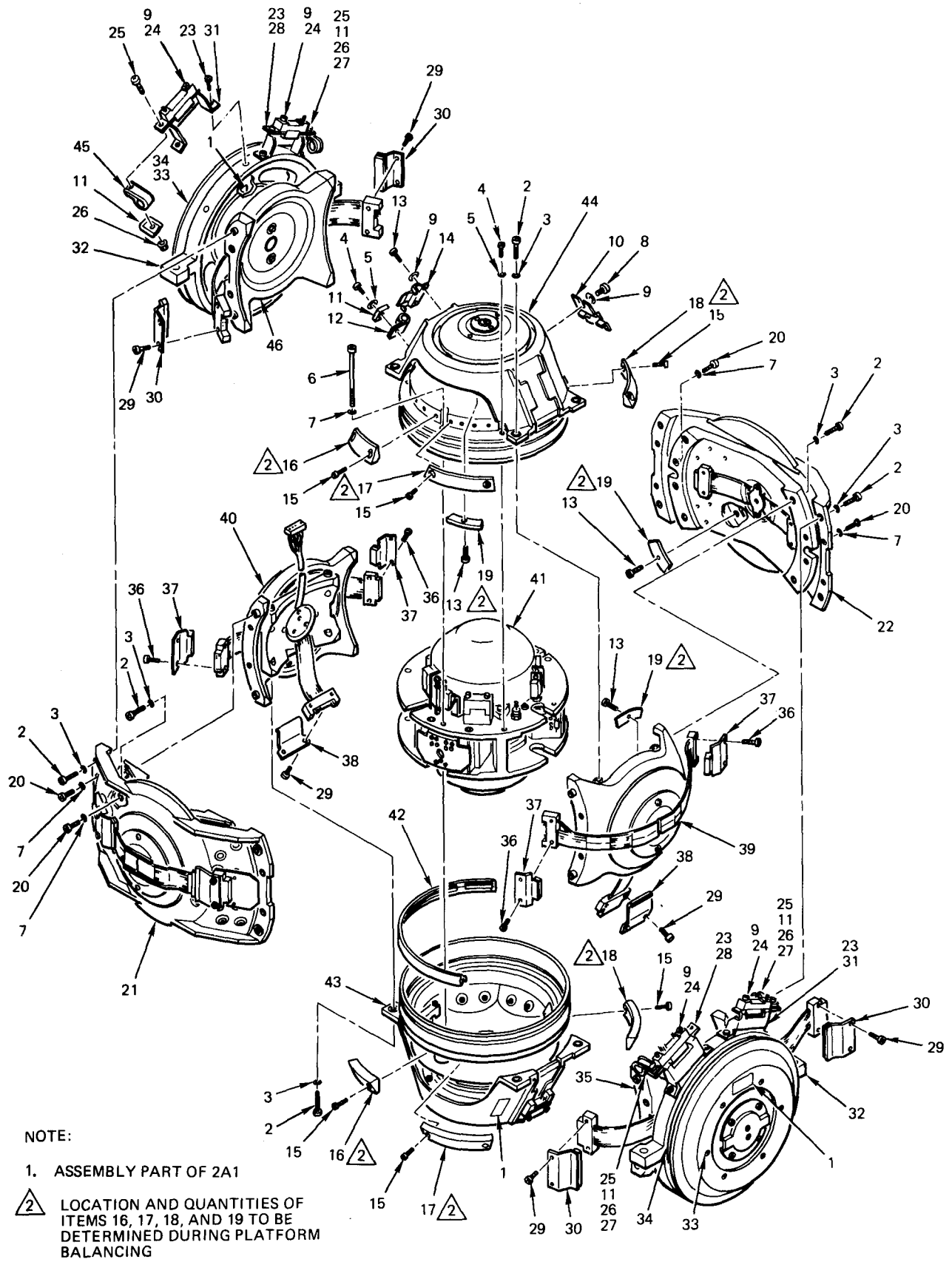
Figure 6. Gimbal Assembly
