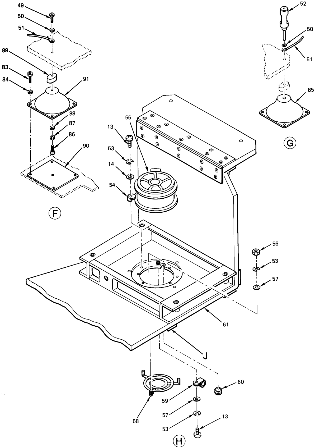
Figure 2. Electrical Equipment Mounting Base (Sheet 3 of 5)
