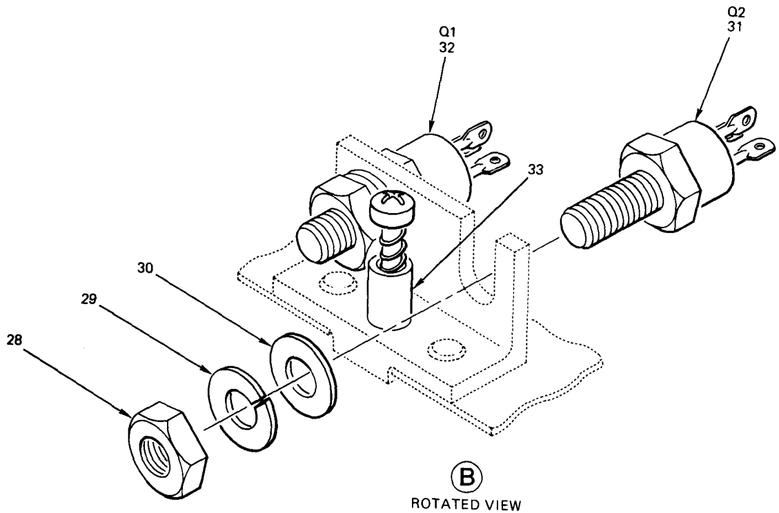
Figure 27. Circuit Card Assembly, \pm 15V Precision Regulator (Sheet 2 of 2)
