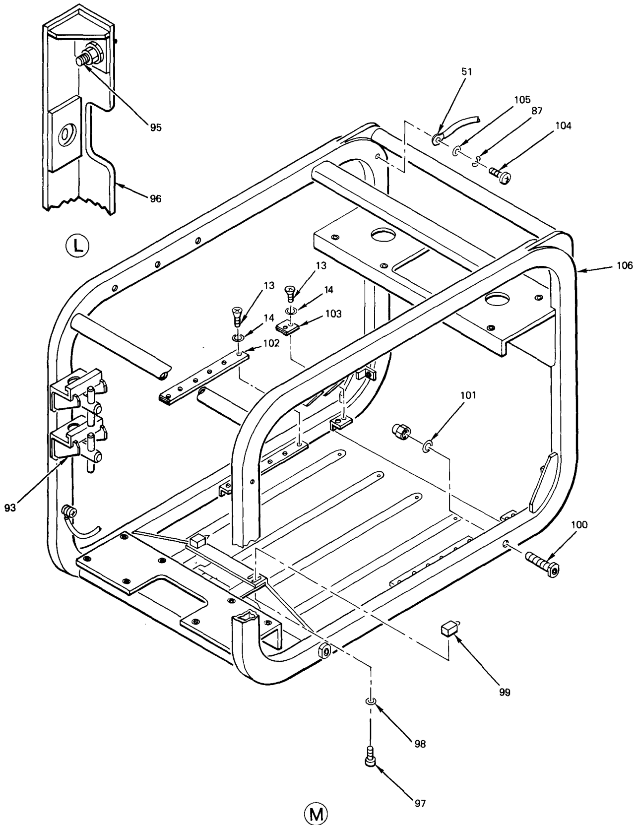
Figure 2. Electrical Equipment Mounting Base (Sheet 5 of 5)
