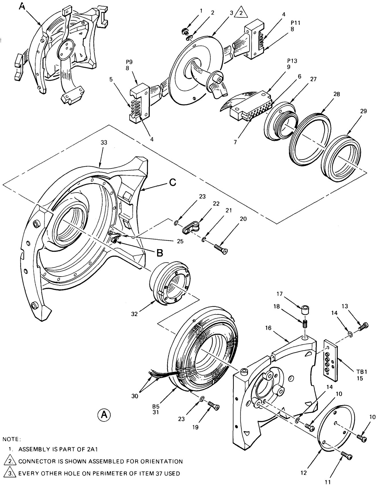
Figure 9. Inner Roll Cartridge Assembly, Resolver (Sheet 1 of 2)
