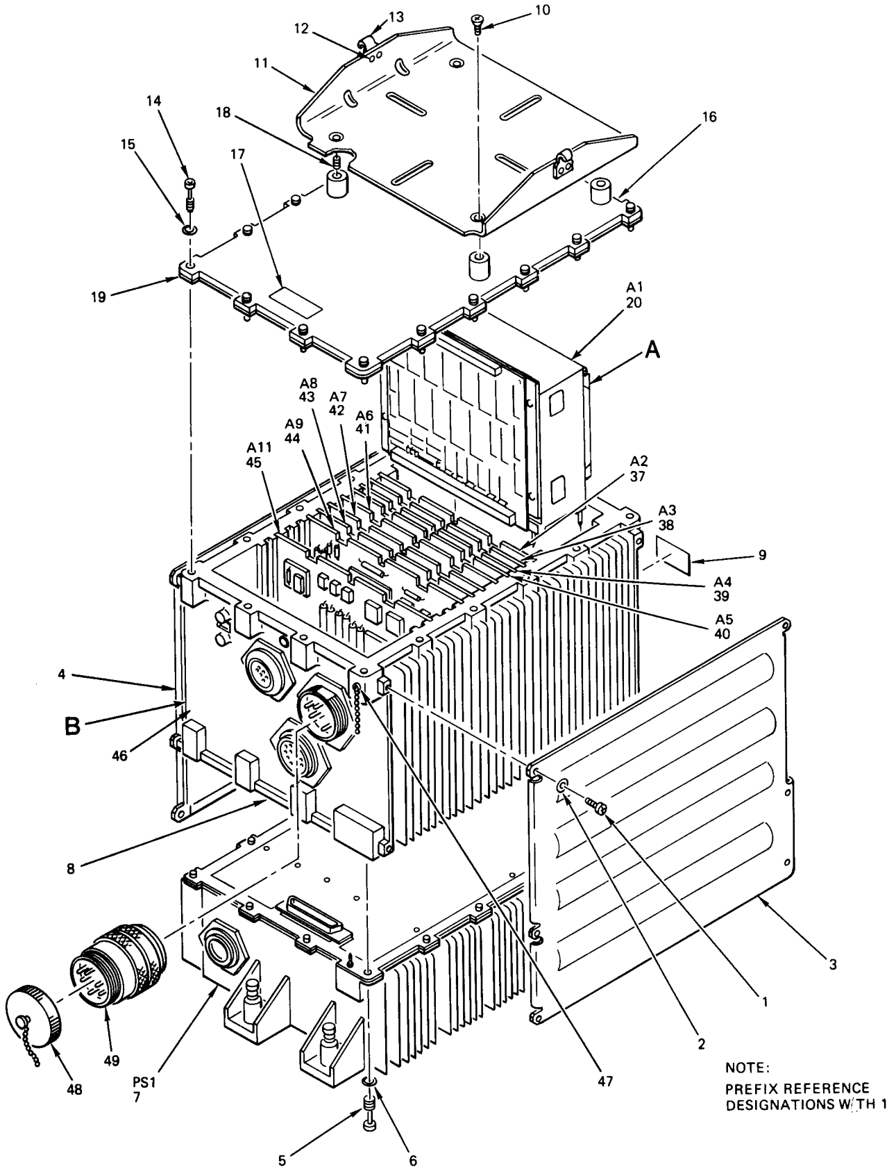
Figure 30. Computer (Sheet 1 of 3)
