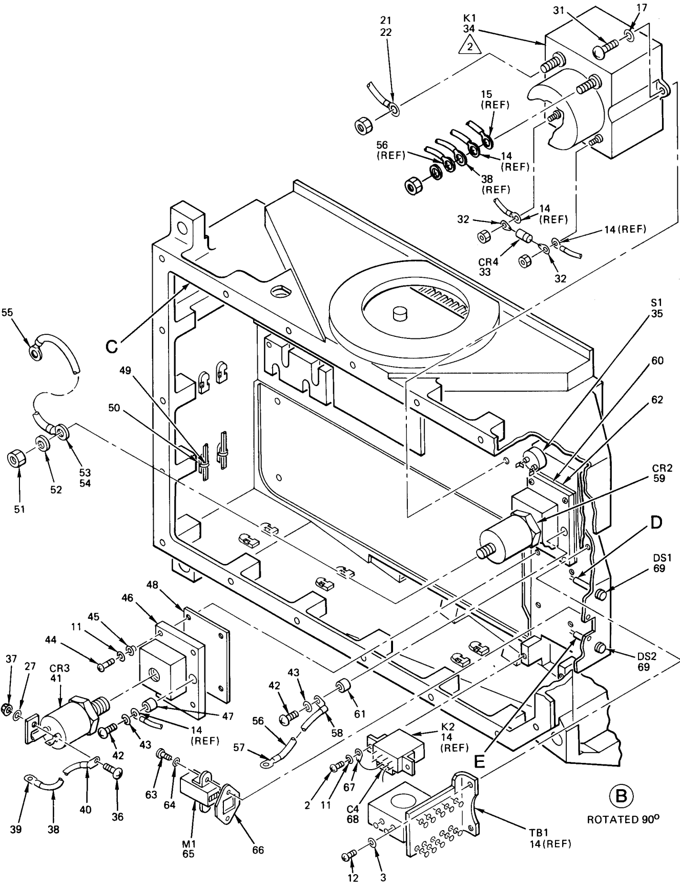
Figure 53. Power Supply Subassembly (Sheet 3 of 6)
