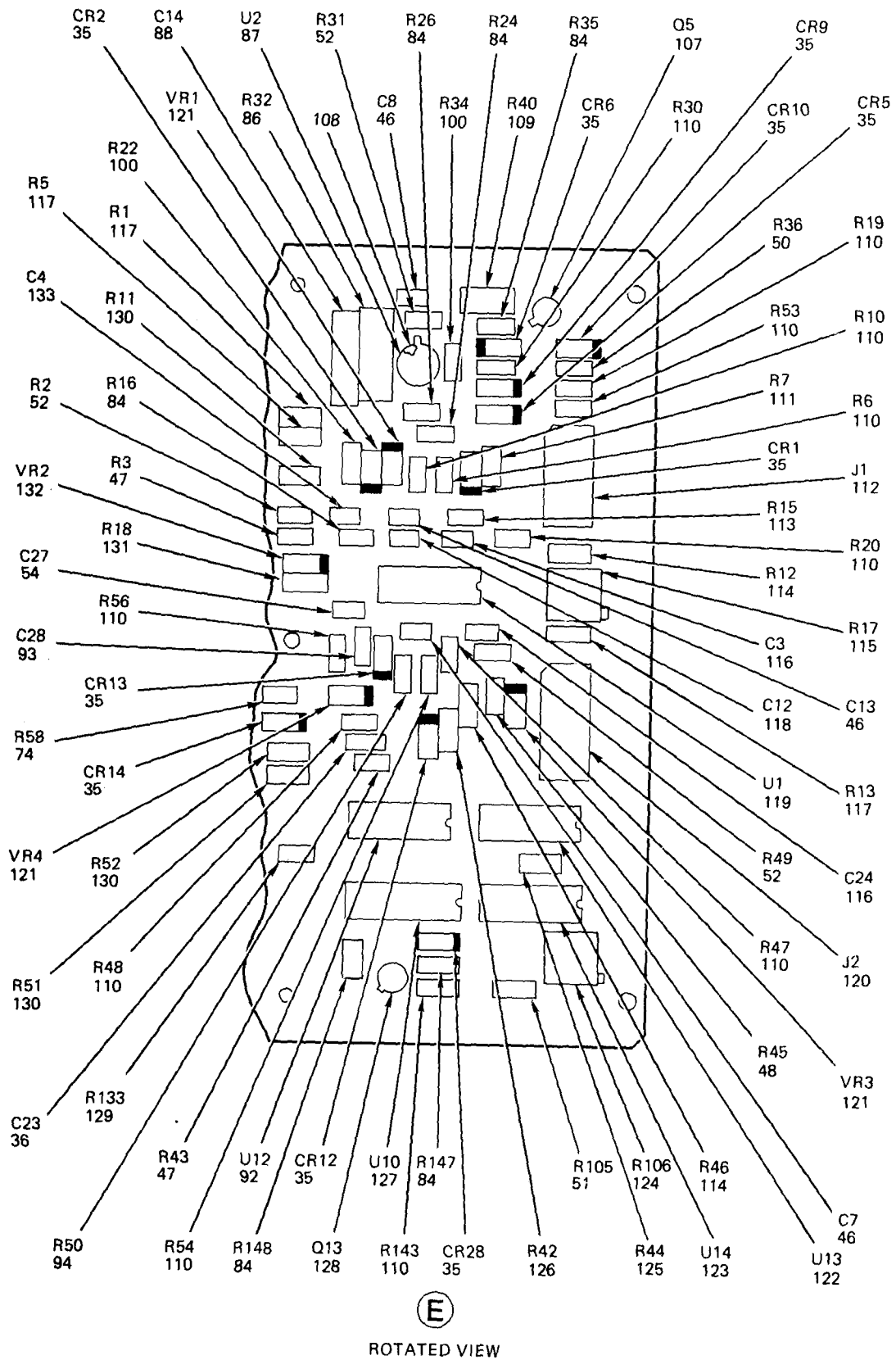
Figure 42. Circuit Card Assembly, 15V (Sheet 4 of 4)
