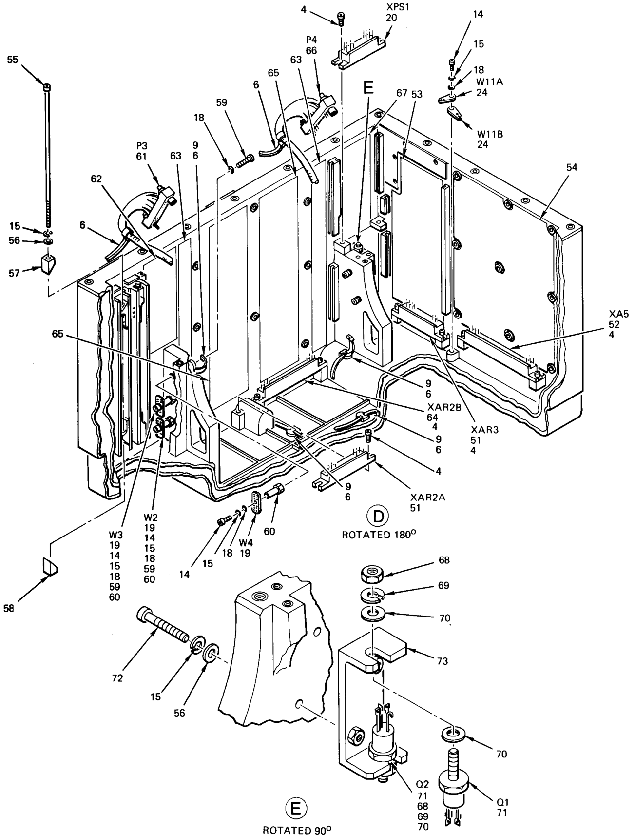
Figure 23. Inertial Measurement Unit Subassembly (Sheet 4 of 6)
