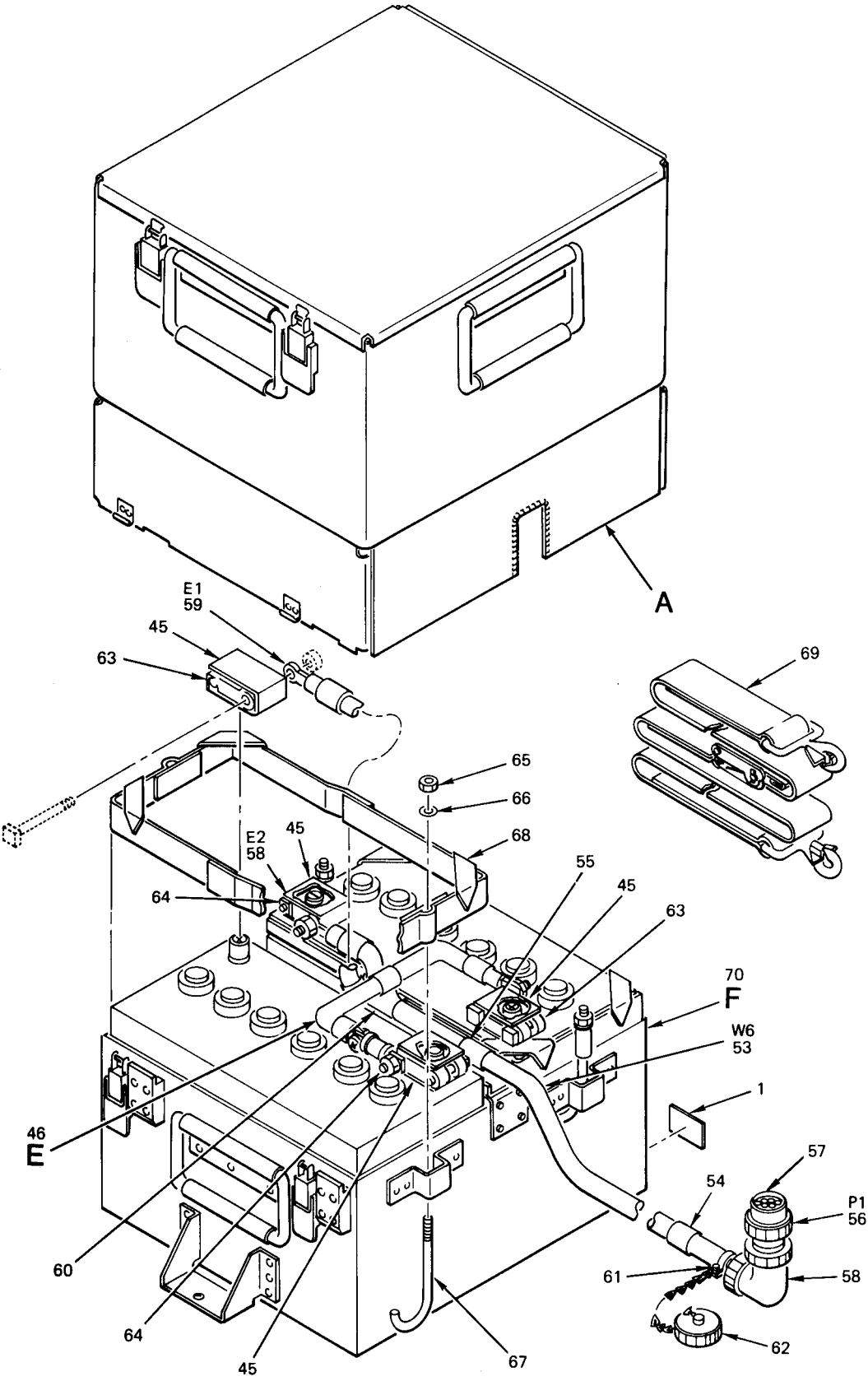
Figure 60. Battery Box (Sheet 1 of 5)
