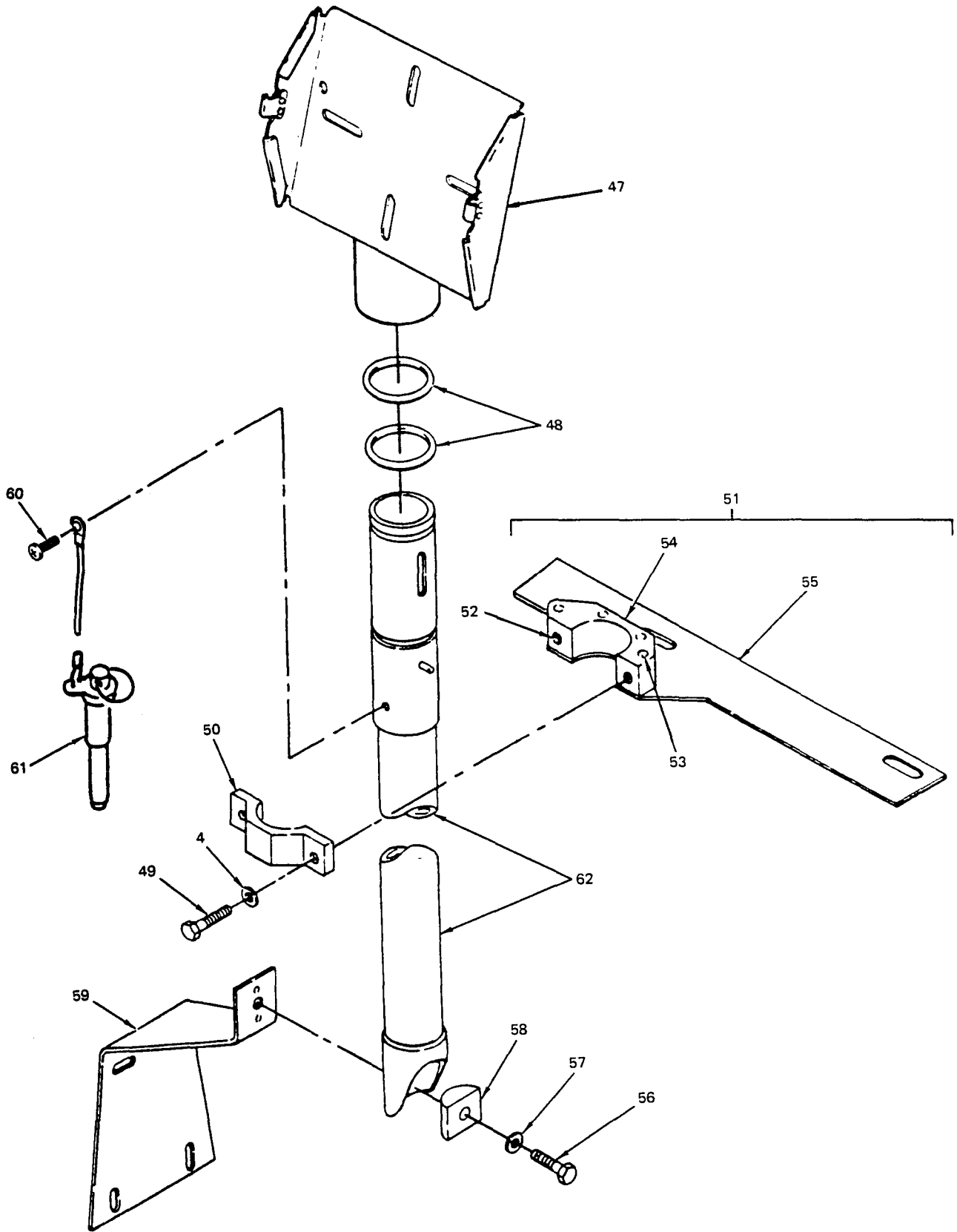
Figure 72. Installation Kit, SUSV (Sheet 3 of 5)
