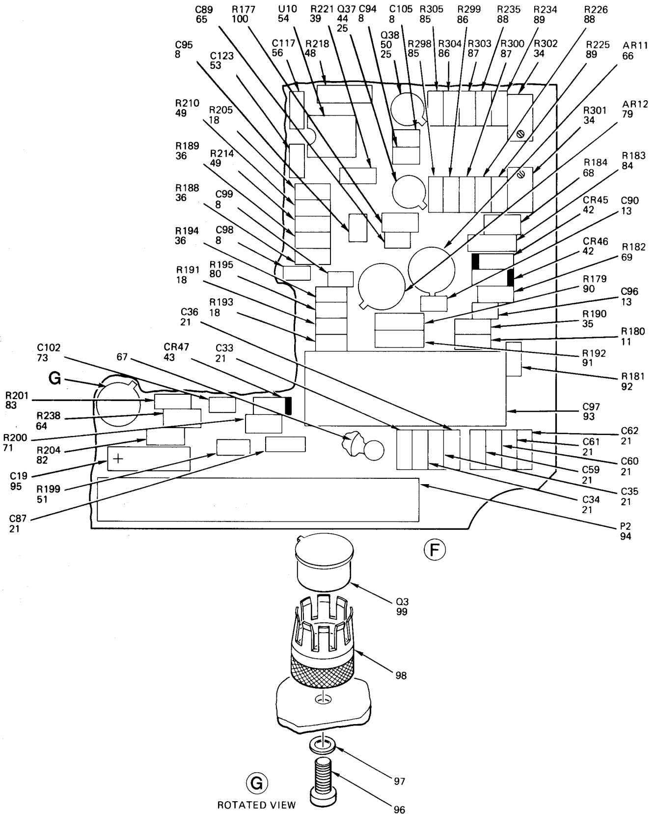
Figure 18. Circuit Card Assembly, Quantizer (Sheet 6 of 8)
