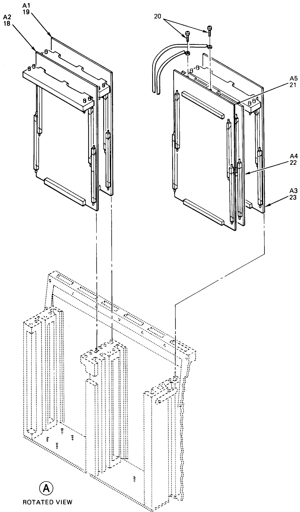
Figure 44. Power Supply (Sheet 2 of 2)
