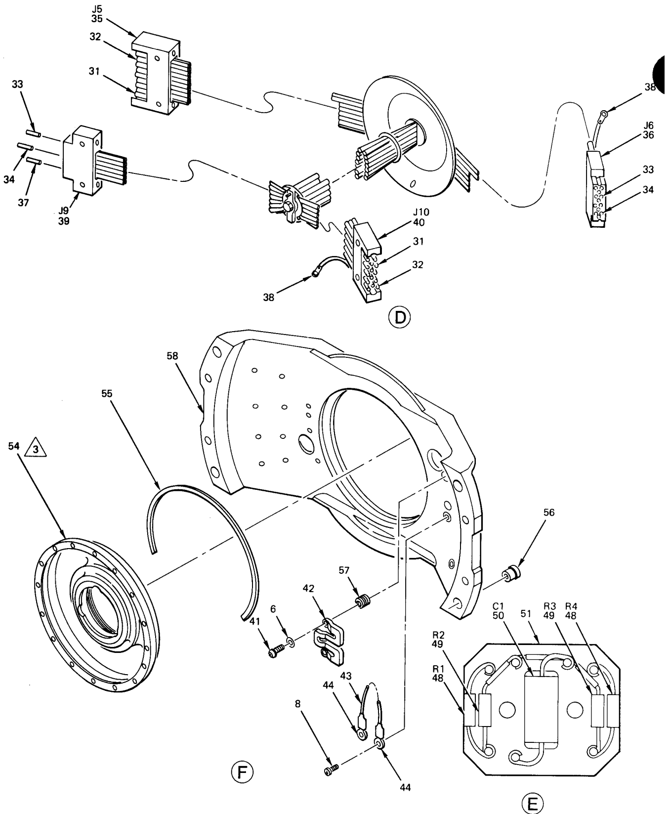
Figure 10. Pitch Cartridge Assembly, Transolver (Sheet 3 of 3)
