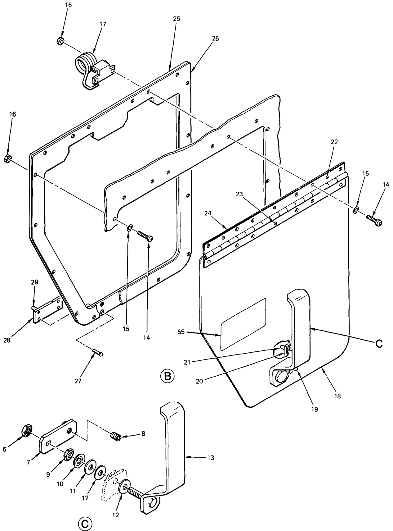
Figure 62. Winterization Kit (Sheet 2 of 4)
