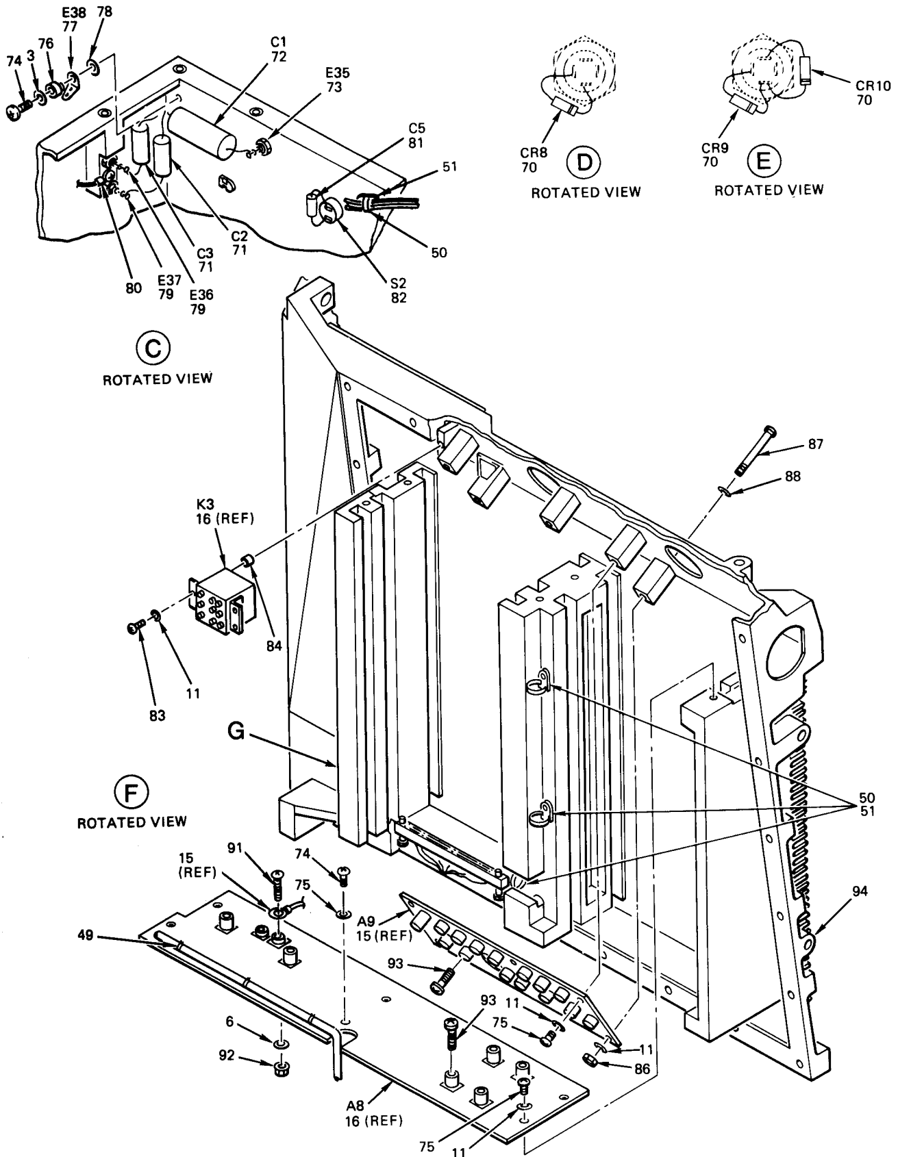
Figure 53. Power Supply Subassembly (Sheet 4 of 6)
