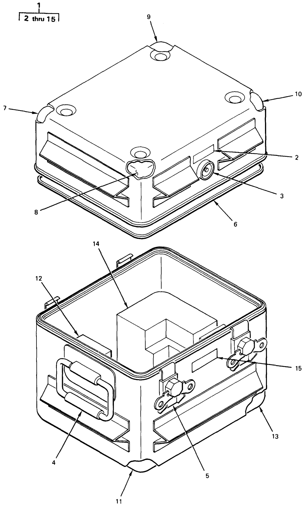
Figure 68. Transit Case, Control and Display
