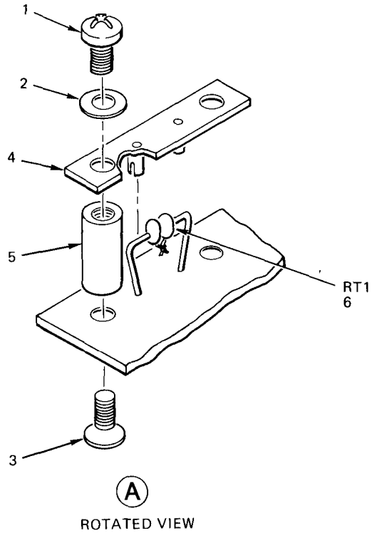
Figure 18. Circuit Card Assembly, Quantizer (Sheet 1 of 8)
